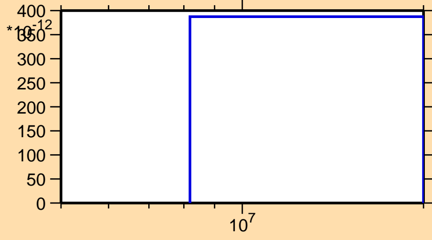
\sigma vs. E for ^{225}\text{Pa}(\text{mt } 45)
