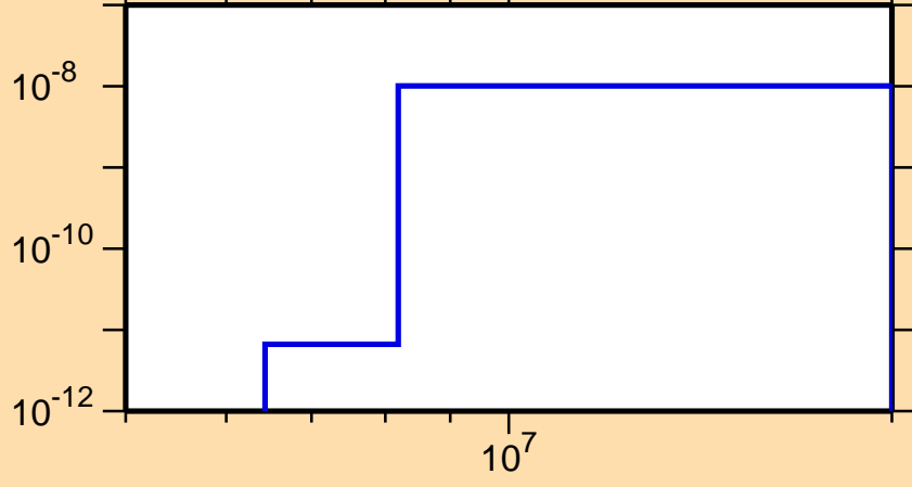
\sigma vs. E for ^{225}\text{Pa}(n,p\alpha)
