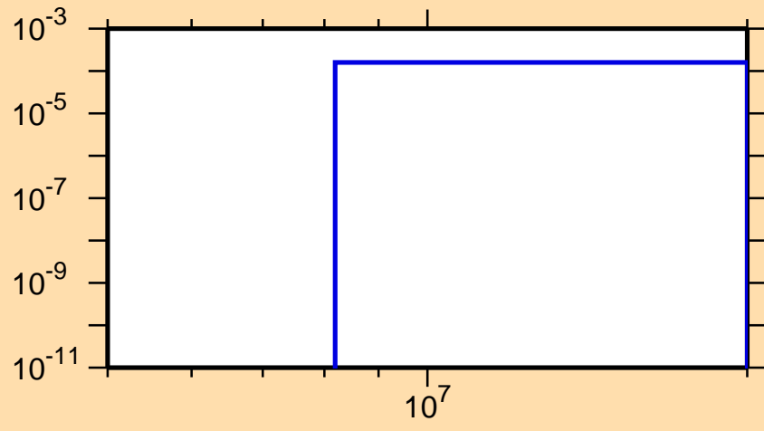
\sigma vs. E for ^{225}\text{Pa}(n,t)
