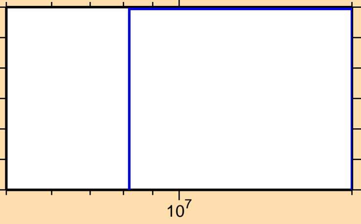
\sigma vs. E for ^{225}\text{Pa}(n,\text{He3})
