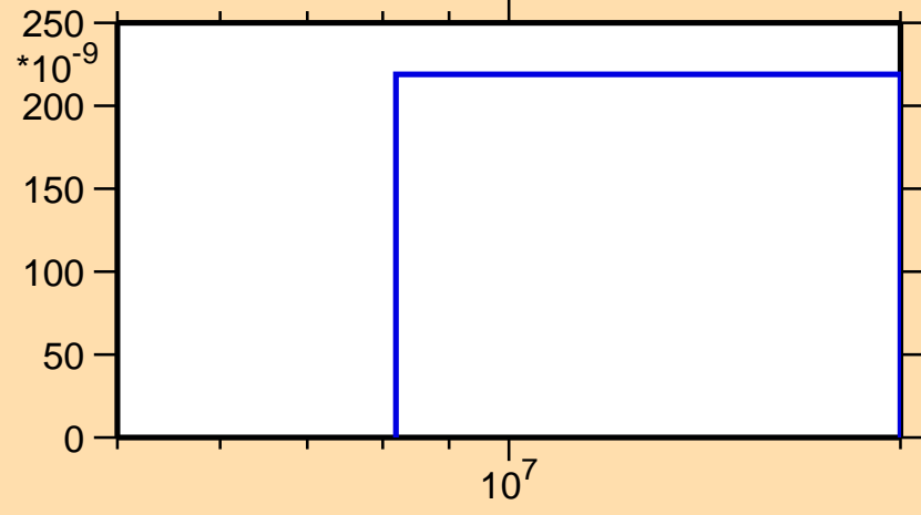
\sigma vs. E for ^{225}\text{Pa}(n,\text{nd})
