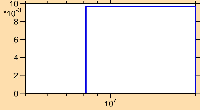
\sigma vs. E for ^{225}\text{Pa}(n,3n)
