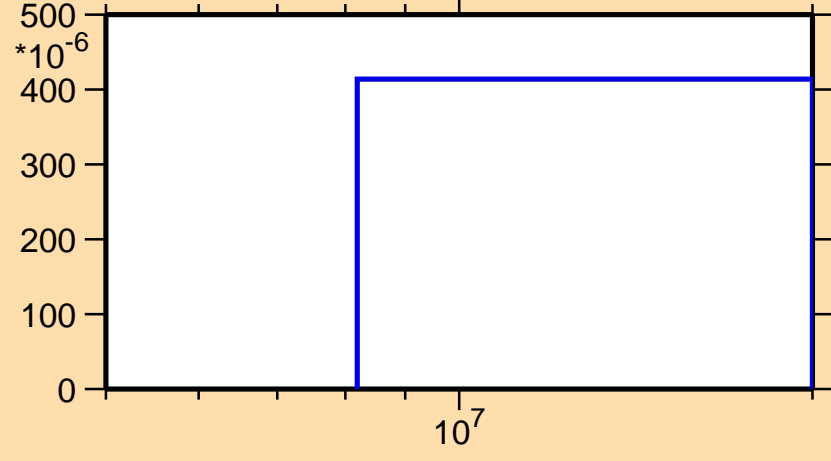
\sigma vs. E for ^{225}\text{Pa}(n,3n\alpha)
