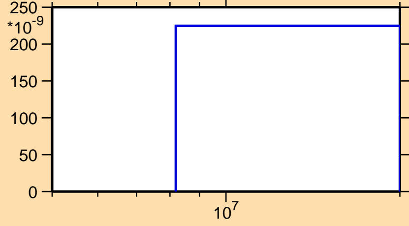
\sigma vs. E for ^{225}\text{Pa}(n,2np)
