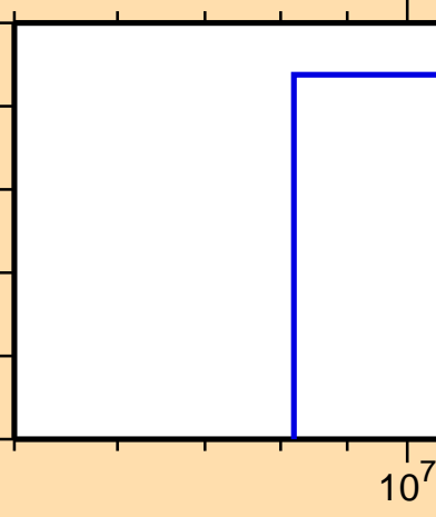
\sigma vs. E for ^{225}\text{Pa} (mt 34)
