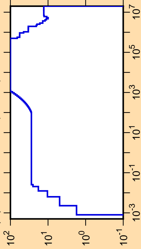
\Delta\mu/\mu vs. E for ^{226}\text{Pa}(\text{mt251})
