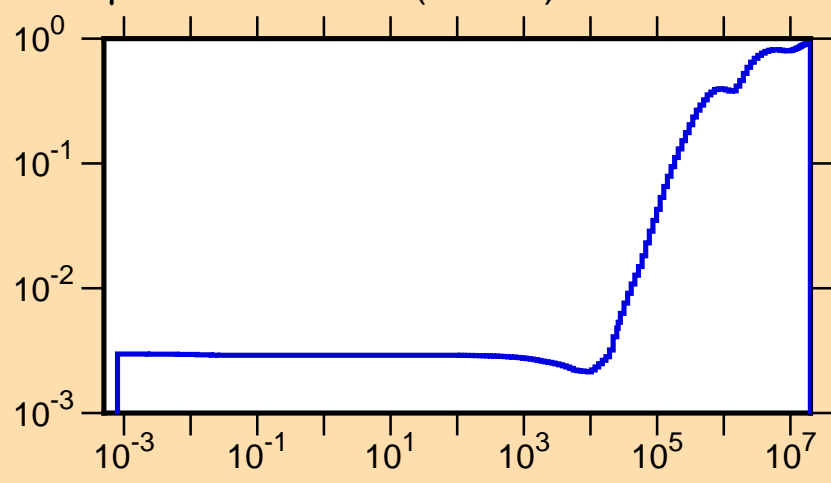
\mu vs. E for ^{226}\text{Pa}(\text{mt251})
