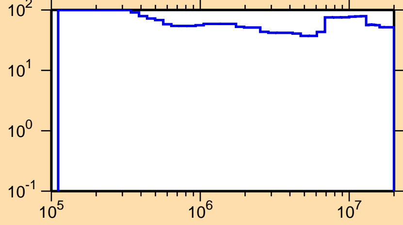
\Delta\sigma/\sigma vs. E for ^{226}\text{Pa}(n,\text{inel.})
