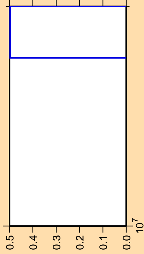
\Delta\sigma/\sigma vs. E for ^{226}\text{Pa} (mt 42)
