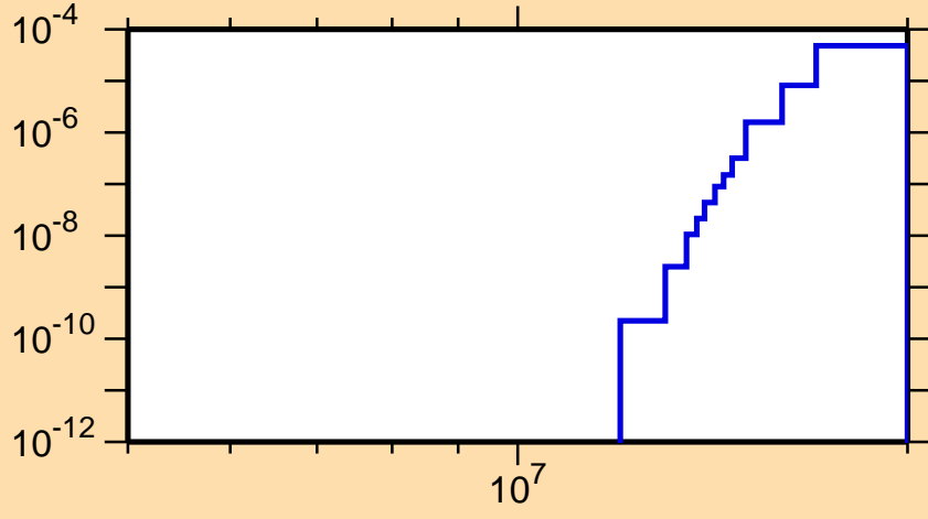
\sigma vs. E for ^{226}\text{Pa}(n,2np)
