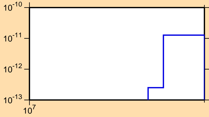
\sigma vs. E for ^{226}\text{Pa} (mt 34)
