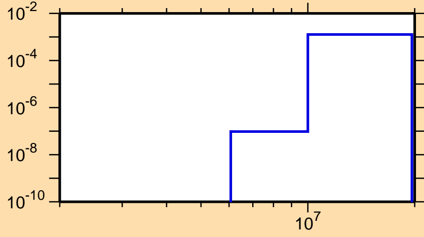
\sigma vs. E for ^{226}\text{Pa}(n,d)
