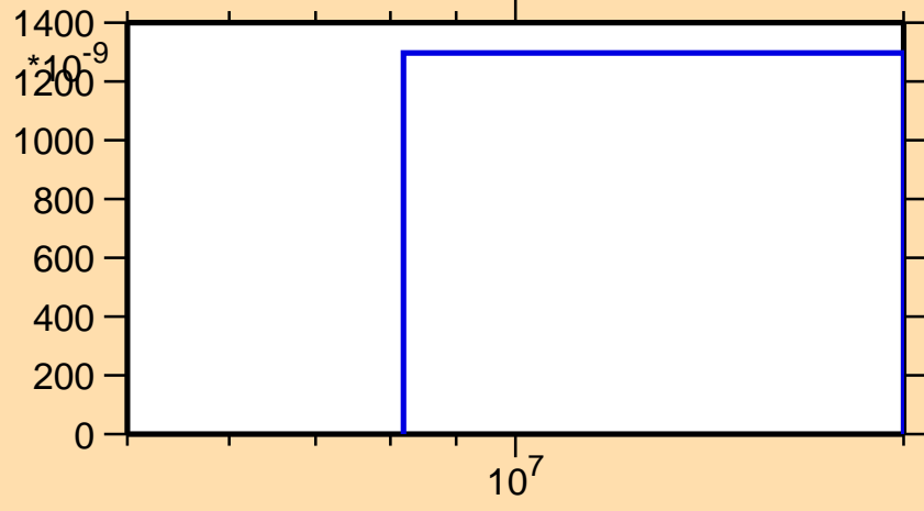
\sigma vs. E for ^{226}\text{Pa}(n,\text{nd})
