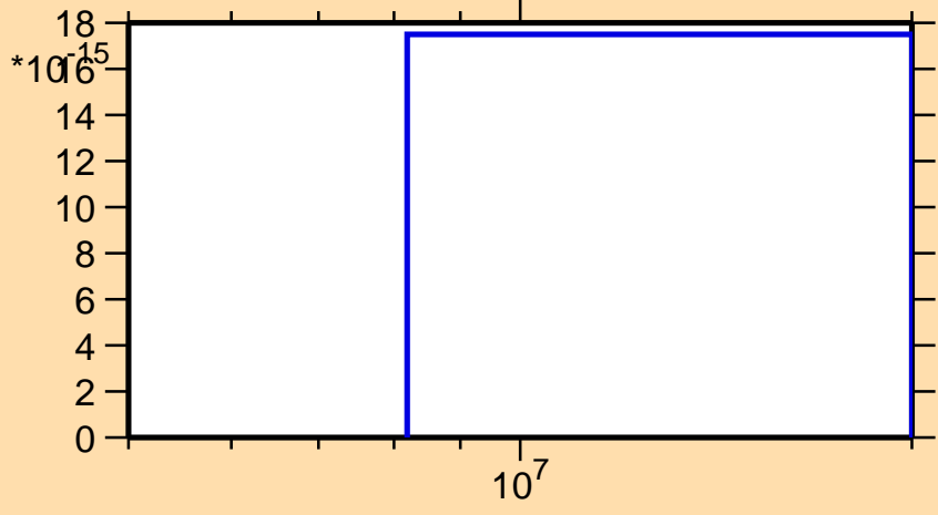
\sigma vs. E for ^{226}\text{Pa} (mt 11)
