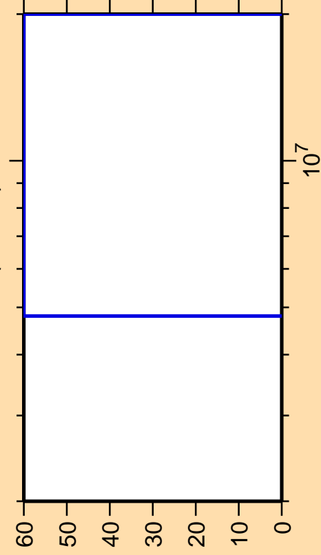
\Delta\sigma/\sigma vs. E for ^{226}\text{Pa}(n,2n\alpha)
