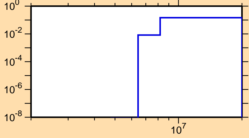
\sigma vs. E for ^{226}\text{Pa}(n,2n\alpha)
