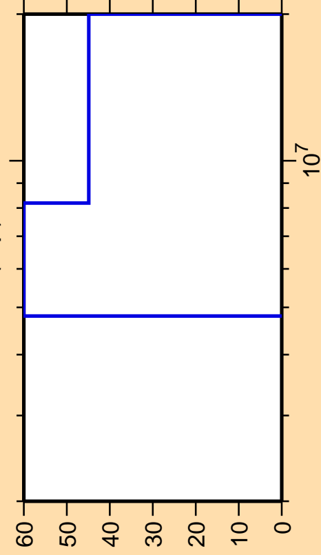
\Delta\sigma/\sigma vs. E for ^{226}\text{Pa}(n,p)
