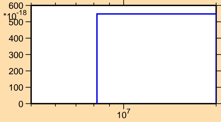
\sigma vs. E for ^{226}\text{Pa} (mt 42)
