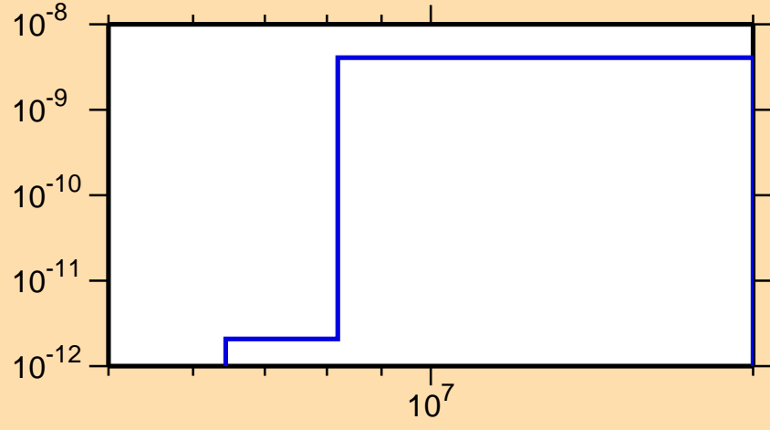
\sigma vs. E for ^{226}\text{Pa}(n,p\alpha)
