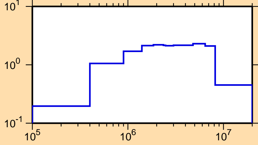
\sigma vs. E for ^{226}\text{Pa}(n,\text{inel.})
