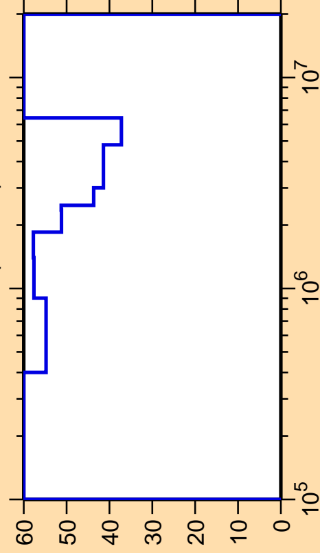
\Delta\sigma/\sigma vs. E for ^{226}\text{Pa}(n,\text{inel.})
