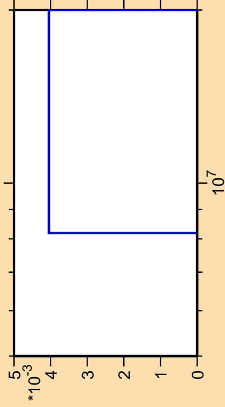
\Delta\sigma/\sigma vs. E for ^{226}\text{Pa} (mt 42)
