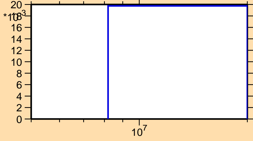
\sigma vs. E for ^{226}\text{Pa}(n,3n)
