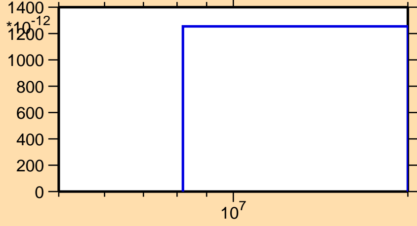
\sigma vs. E for ^{226}\text{Pa}(n,\text{He3})
