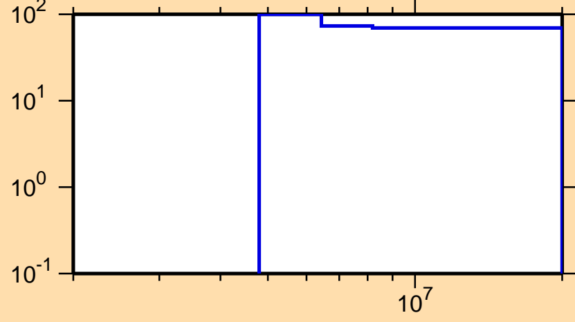
\Delta\sigma/\sigma vs. E for ^{226}\text{Pa}(n,2n)
