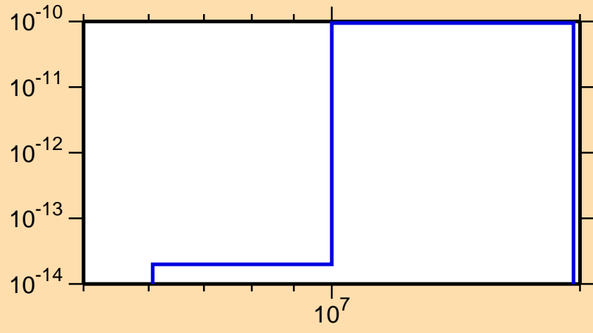
\sigma vs. E for ^{227}\text{Pa}(n,p\alpha)
