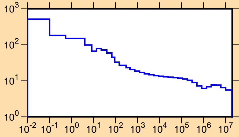
\sigma vs. E for ^{227}\text{Pa}(n,\text{tot.})
