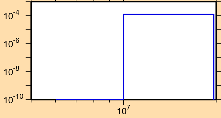
\sigma vs. E for ^{227}\text{Pa}(n,t)
