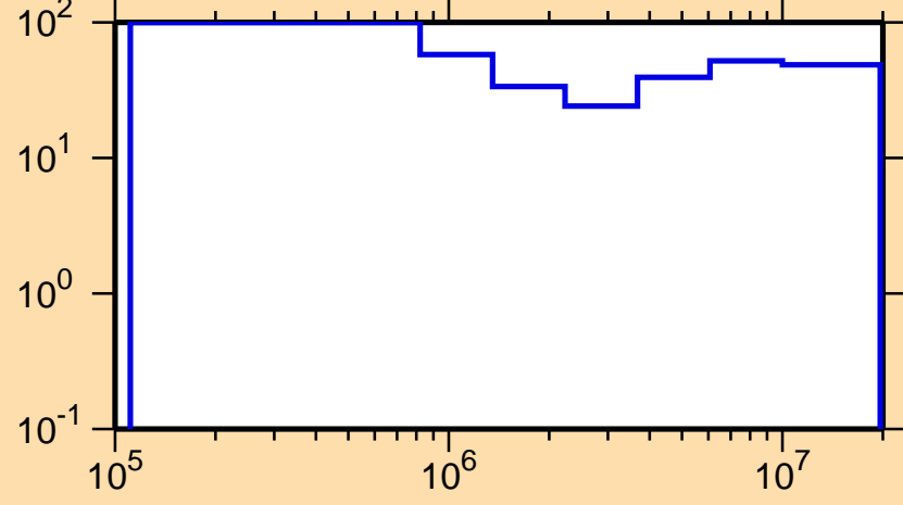
\Delta\sigma/\sigma vs. E for ^{227}\text{Pa}(n,n\text{cont.})
