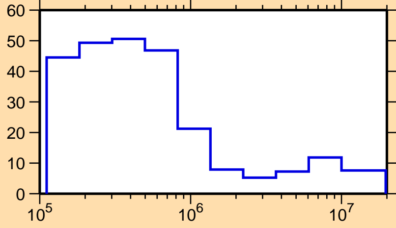
\Delta\sigma/\sigma vs. E for ^{227}\text{Pa}(n,tot.)
