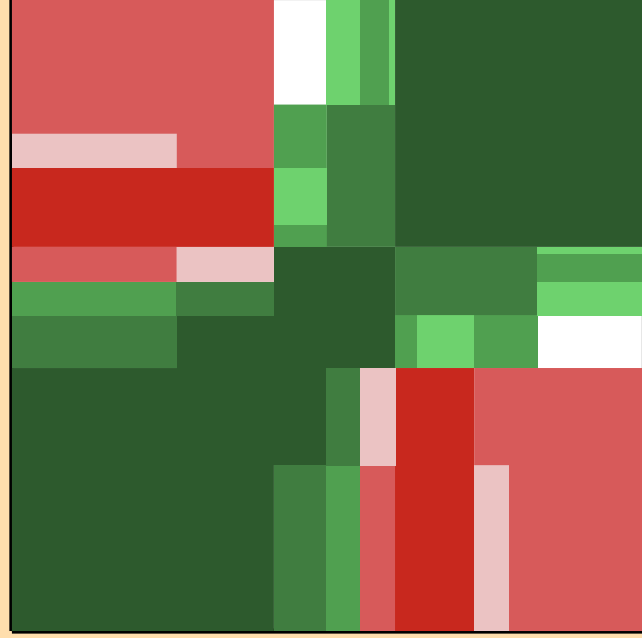
\sigma vs. E for ^{227}\text{Pa}(n,\text{inel.})
