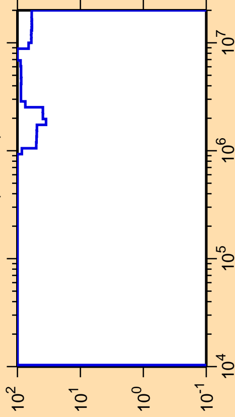
\Delta\sigma/\sigma vs. E for ^{229}\text{Pa}(n,\text{inel.})
