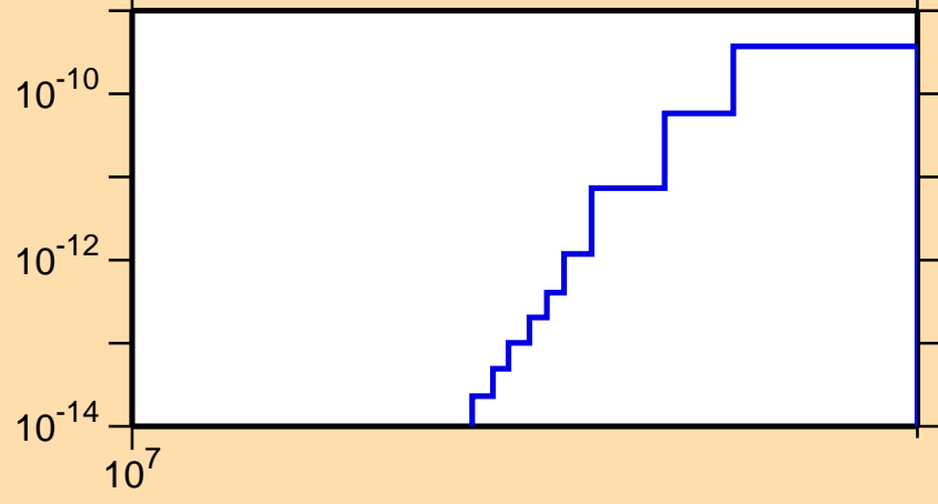
\sigma vs. E for ^{229}\text{Pa}(\text{mt117})
