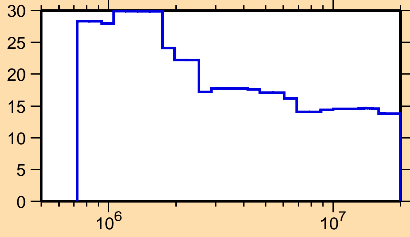
\Delta\sigma/\sigma vs. E for ^{229}\text{Pa}(n,n\text{nonel.})
