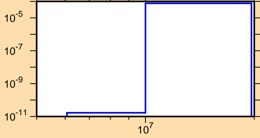
\sigma vs. E for ^{229}\text{Pa}(n,t)
