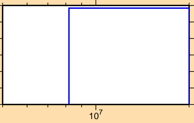
\sigma vs. E for ^{229}\text{Pa}(n,\text{nd})
