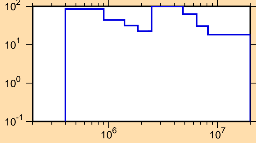
\Delta\sigma/\sigma vs. E for ^{229}\text{Pa}(n,f)
