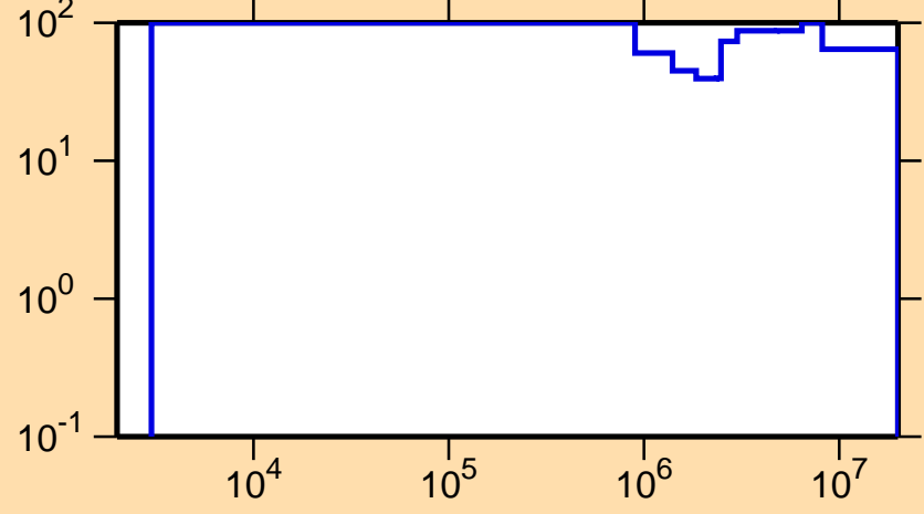
\Delta\sigma/\sigma vs. E for ^{229}\text{Pa}(n,\text{inel.})
