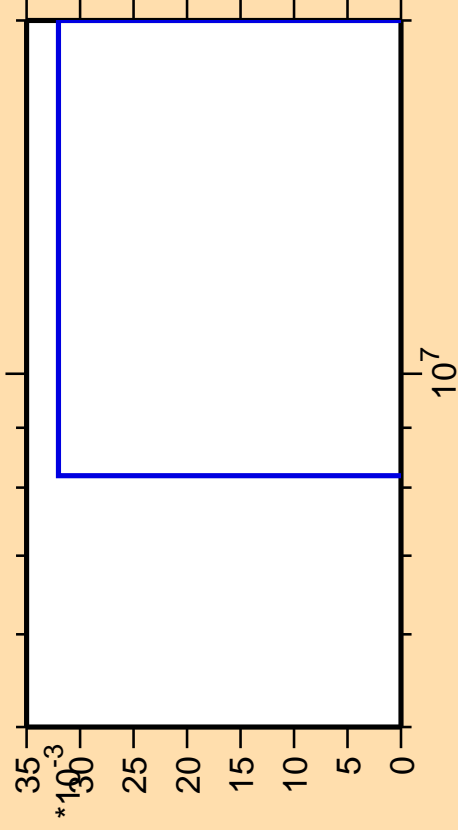
\Delta\sigma/\sigma vs. E for ^{229}\text{Pa} (mt 11)
