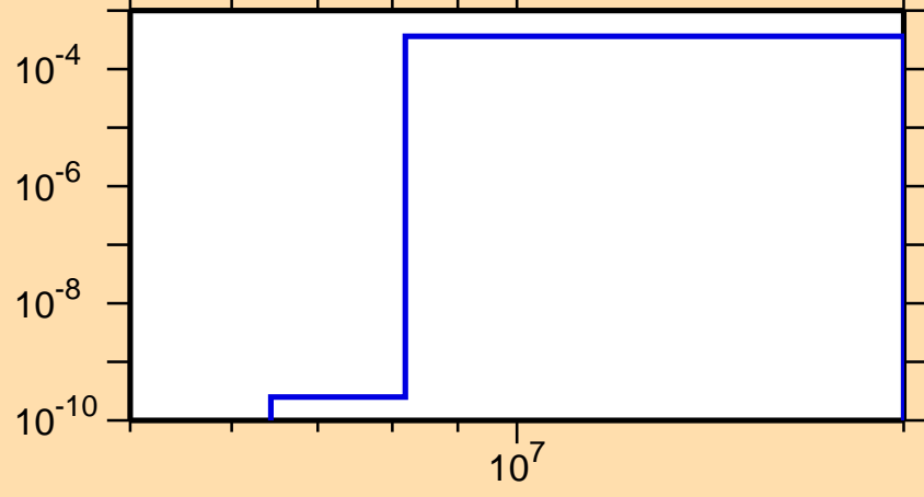
\sigma vs. E for ^{229}\text{Pa}(n,d)
