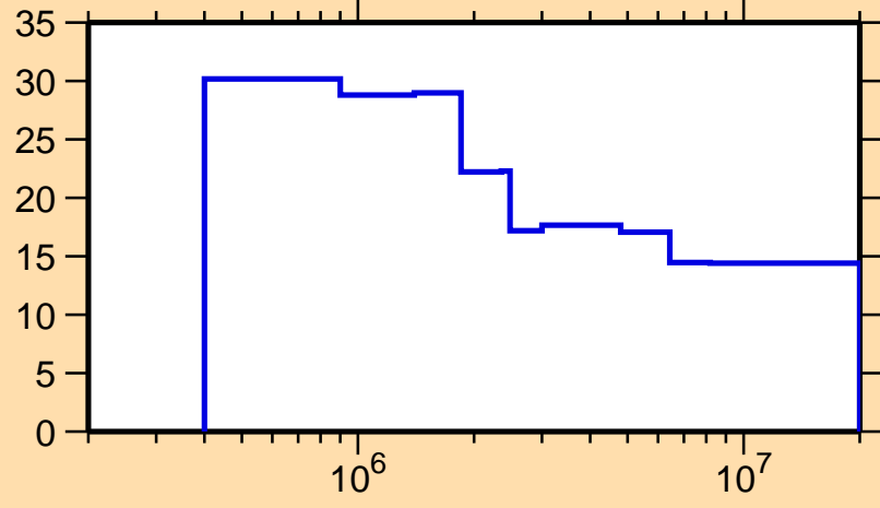
\Delta\sigma/\sigma vs. E for ^{229}\text{Pa}(n,n\text{onel.})
