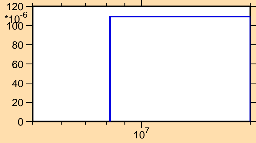
\sigma vs. E for ^{229}\text{Pa}(n,3n)
