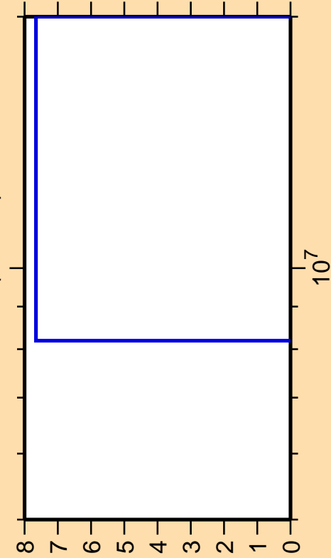
\Delta\sigma/\sigma vs. E for ^{229}\text{Pa}(n,3n\alpha)
