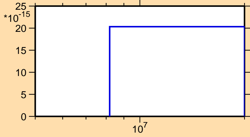
\sigma vs. E for ^{229}\text{Pa} (mt 11)
