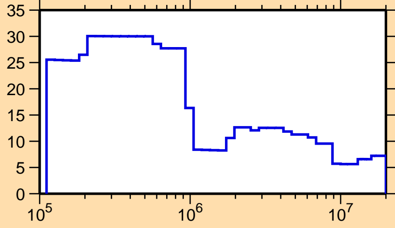
\Delta\sigma/\sigma vs. E for ^{230}\text{Pa}(n, tot.)
