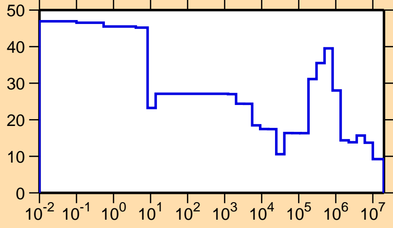
\Delta\sigma/\sigma vs. E for ^{230}\text{Pa}(n,el.)
