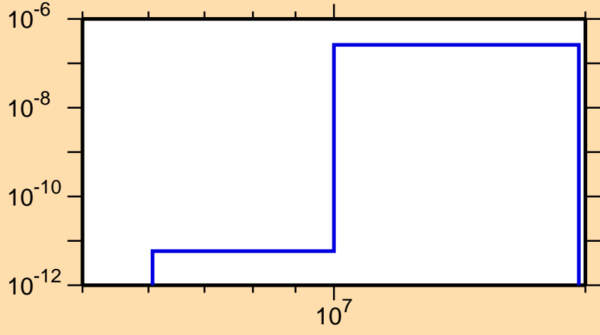
\sigma vs. E for ^{230}\text{Pa}(n,2n\alpha)
