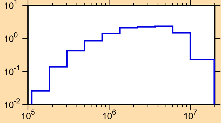
\sigma vs. E for ^{230}\text{Pa}(n,\text{inel.})
