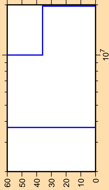
\Delta\sigma/\sigma vs. E for ^{230}\text{Pa}(n,f)
