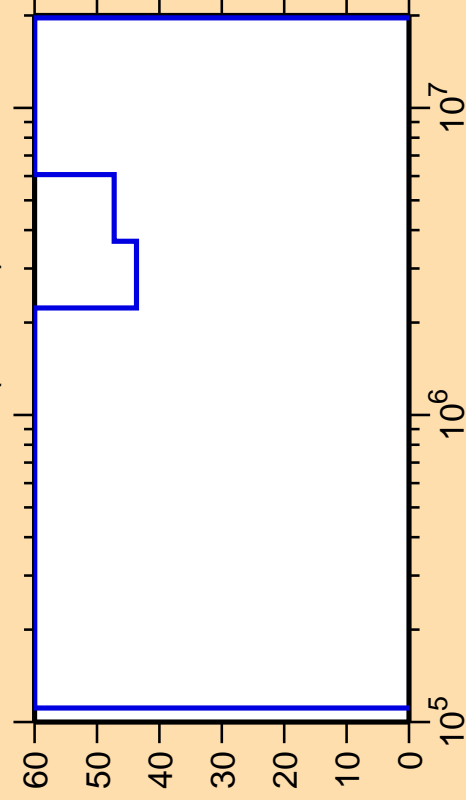
\Delta\sigma/\sigma vs. E for ^{230}\text{Pa}(n,\text{inel.})
