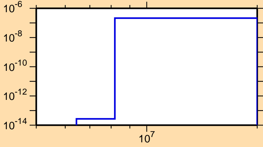
\sigma vs. E for ^{230}\text{Pa}(n,2n\alpha)
