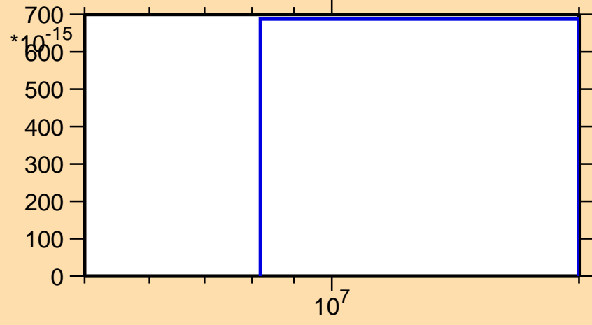
\sigma vs. E for ^{230}\text{Pa}(n,3n\alpha)
