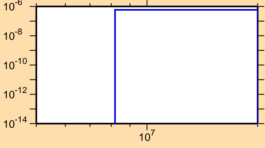
\sigma vs. E for ^{230}\text{Pa}(n,\text{nd})
