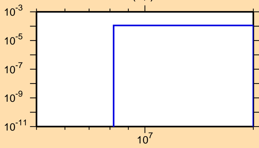
\sigma vs. E for ^{230}\text{Pa}(n,t)
