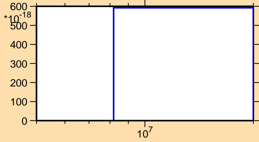
\sigma vs. E for ^{230}\text{Pa} (mt 34)
