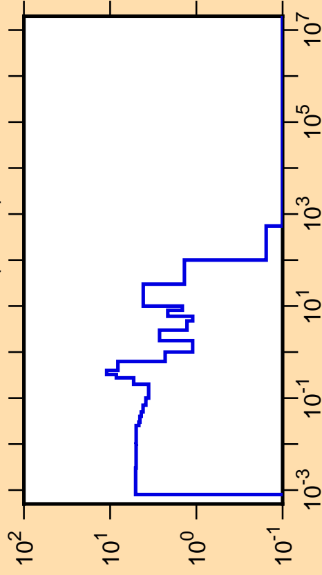
\Delta\sigma/\sigma vs. E for ^{231}\text{Pa}(n,\text{tot.})
