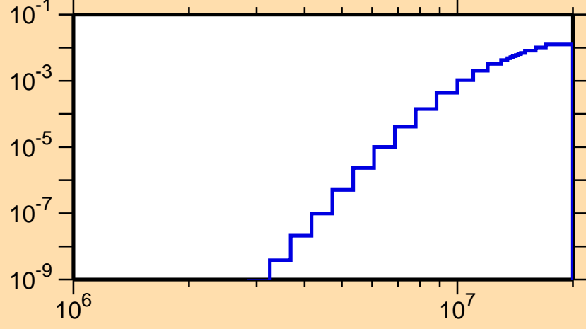
\sigma vs. E for ^{232}\text{Pa}(n,p)
