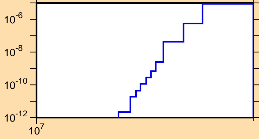
\sigma vs. E for ^{232}\text{Pa}(n,nt)
