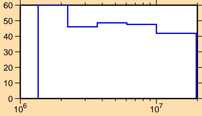
\Delta\sigma/\sigma vs. E for ^{232}\text{Pa}(n,n\text{cont.})
