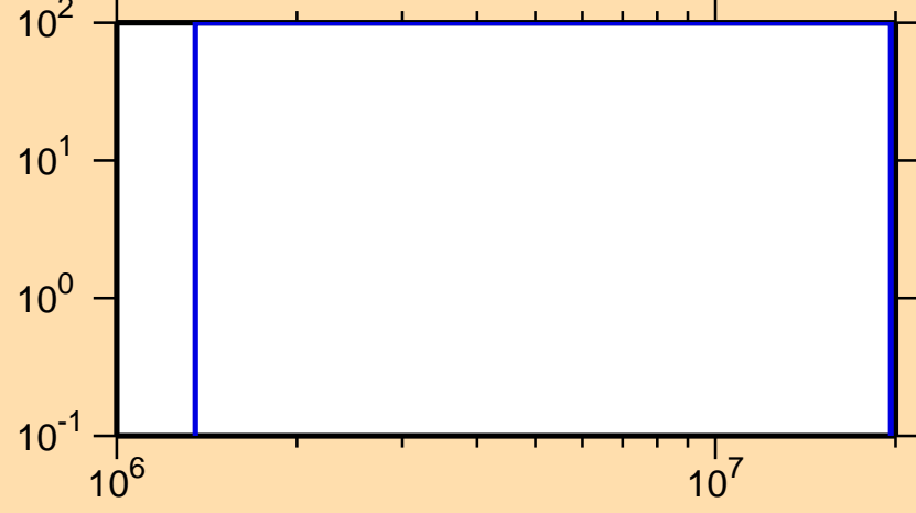
\Delta\sigma/\sigma vs. E for ^{232}\text{Pa}(n,n_1)
