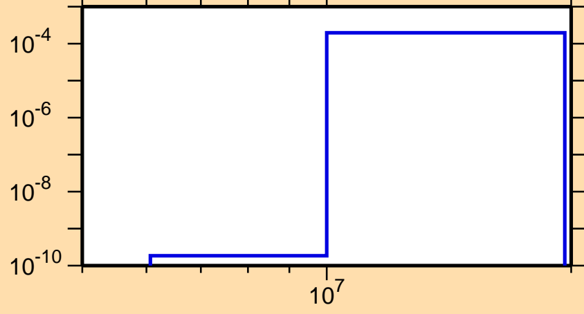
\sigma vs. E for ^{232}\text{Pa}(n,np)
