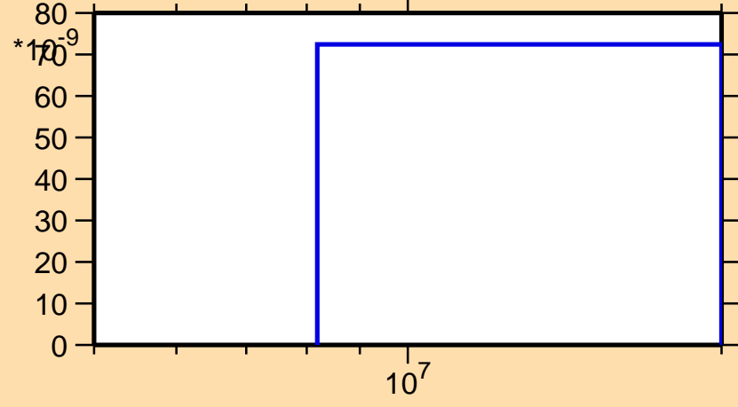
\sigma vs. E for ^{232}\text{Pa}(n,2n\alpha)
