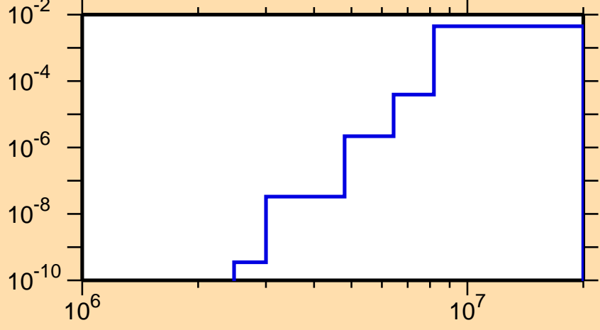
\sigma vs. E for ^{232}\text{Pa}(n,p)
