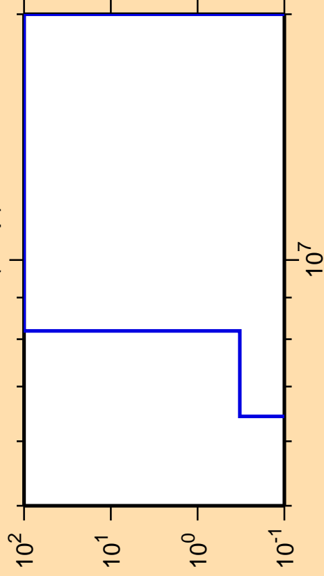
\Delta\sigma/\sigma vs. E for ^{232}\text{Pa}(n,np)
