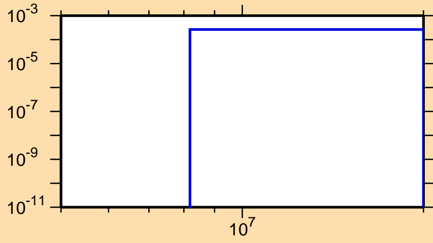
\sigma vs. E for ^{232}\text{Pa}(n,d)
