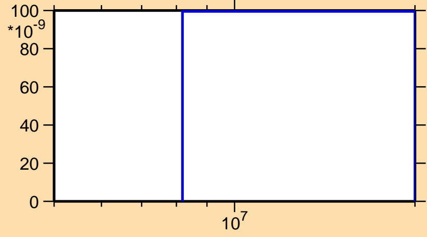
\sigma vs. E for ^{232}\text{Pa}(n,\text{nt})
