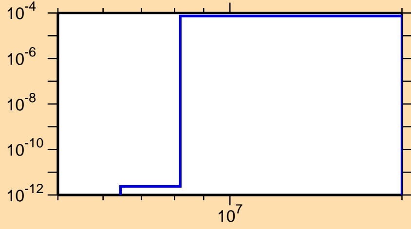
\sigma vs. E for ^{232}\text{Pa}(n,t)
