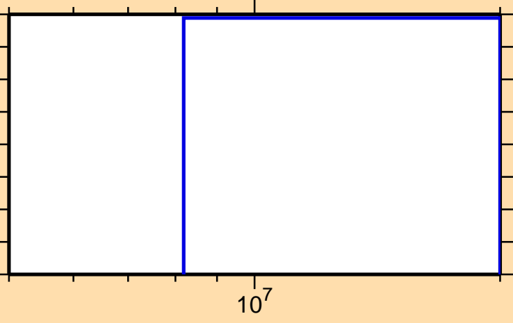
\sigma vs. E for ^{232}\text{Pa}(n,3n\alpha)
