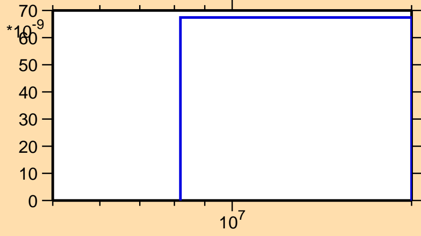
\sigma vs. E for ^{232}\text{Pa}(n,2np)
