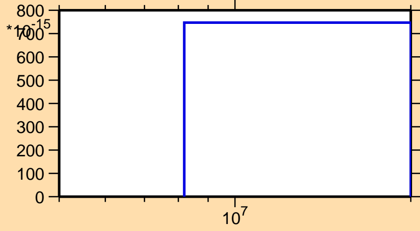
\sigma vs. E for ^{232}\text{Pa}(n,\text{He3})
