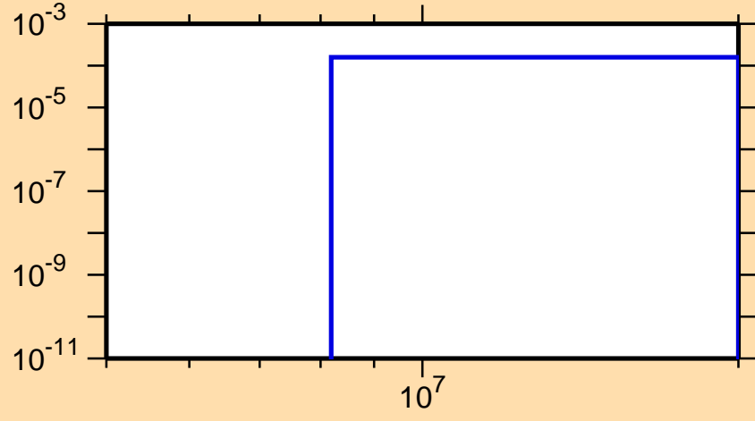
\sigma vs. E for ^{232}\text{Pa}(n,np)
