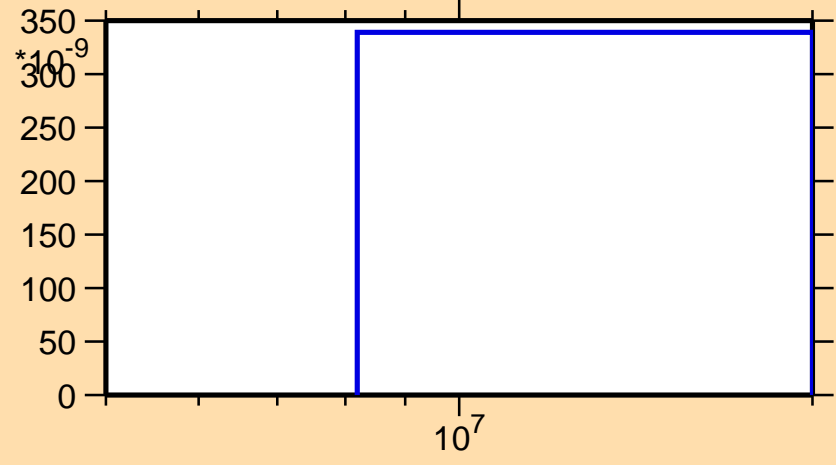
\sigma vs. E for ^{232}\text{Pa}(n,\text{nd})
