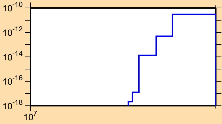
\sigma vs. E for ^{233}\text{Pa}(n,3n\alpha)
