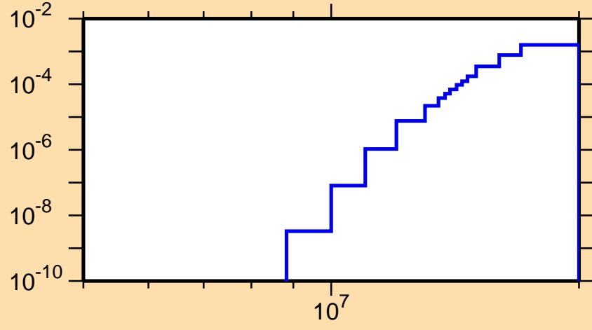
\sigma vs. E for ^{233}\text{Pa}(n,d)
