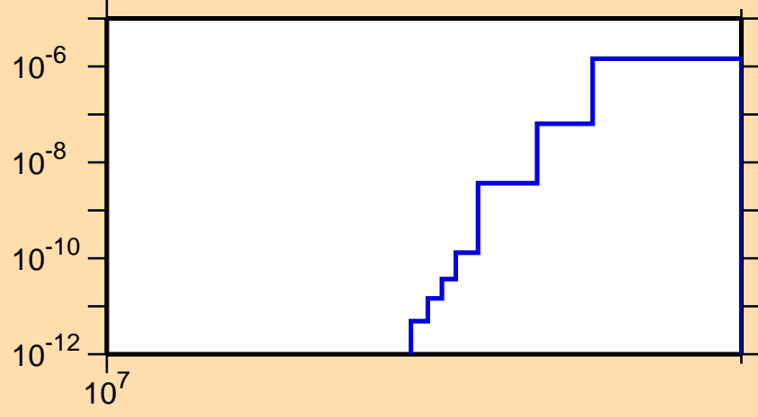
\sigma vs. E for ^{233}\text{Pa}(n,\text{nd})
