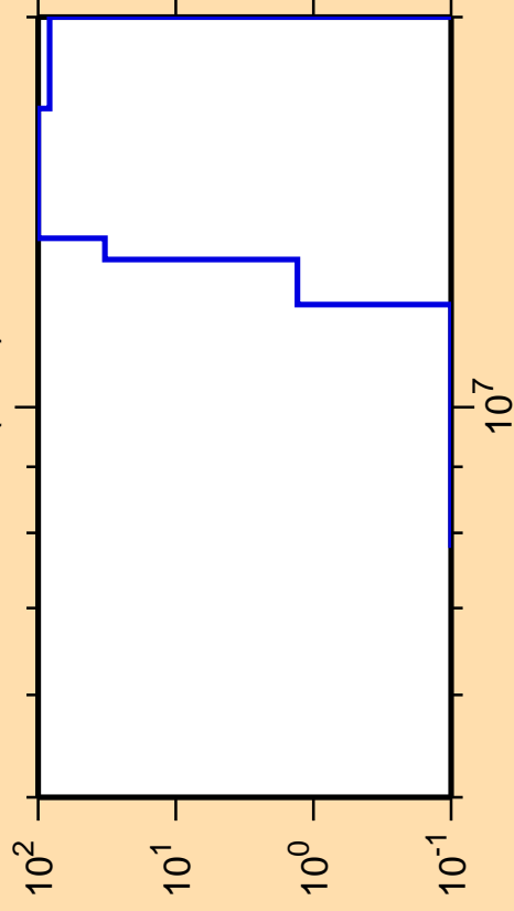
\Delta\sigma/\sigma vs. E for ^{233}\text{Pa}(n,\text{nt})
