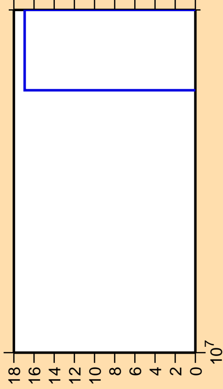
\Delta\sigma/\sigma vs. E for ^{233}\text{Pa}(n,\text{He3})
