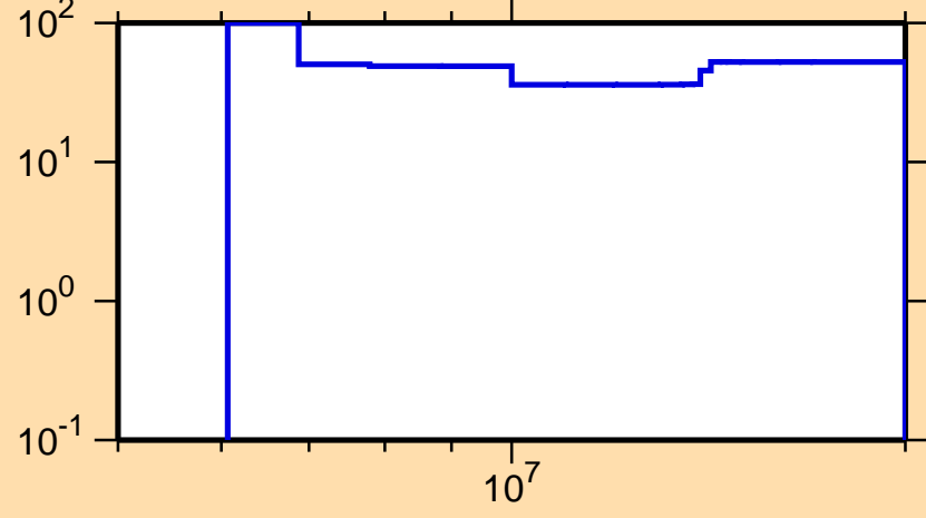
\Delta\sigma/\sigma vs. E for ^{233}\text{Pa}(n,2n)
