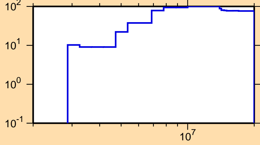
\Delta\sigma/\sigma vs. E for ^{233}\text{Pa}(n,\text{inel.})
