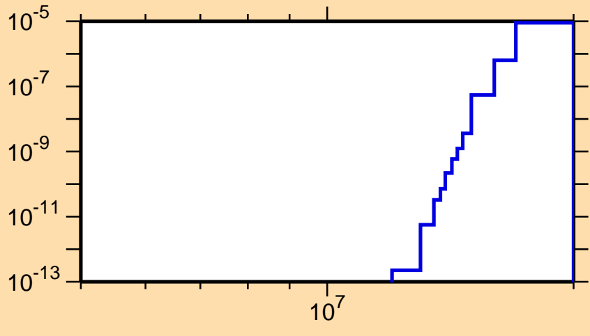
\sigma vs. E for ^{233}\text{Pa}(n,\text{nt})
