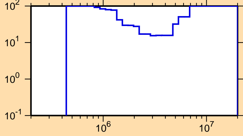
\Delta\sigma/\sigma vs. E for ^{233}\text{Pa}(n,n\text{cont.})
