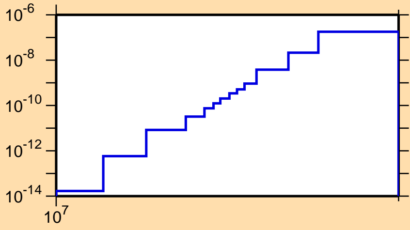
\sigma vs. E for ^{233}\text{Pa}(n,2n\alpha)
