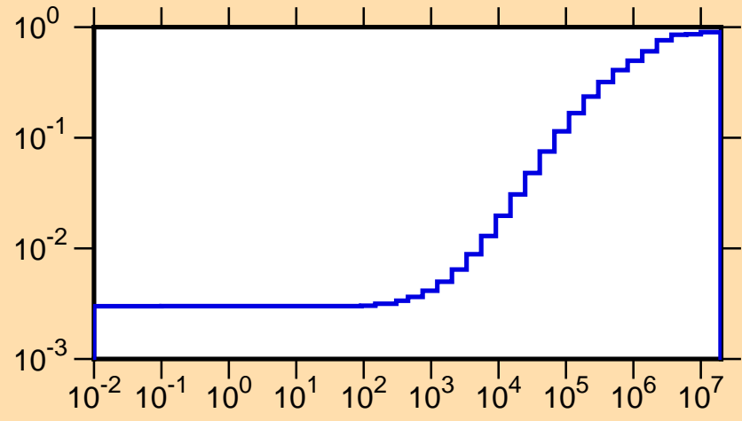
\mu vs. E for ^{233}\text{Pa}(\text{mt251})
