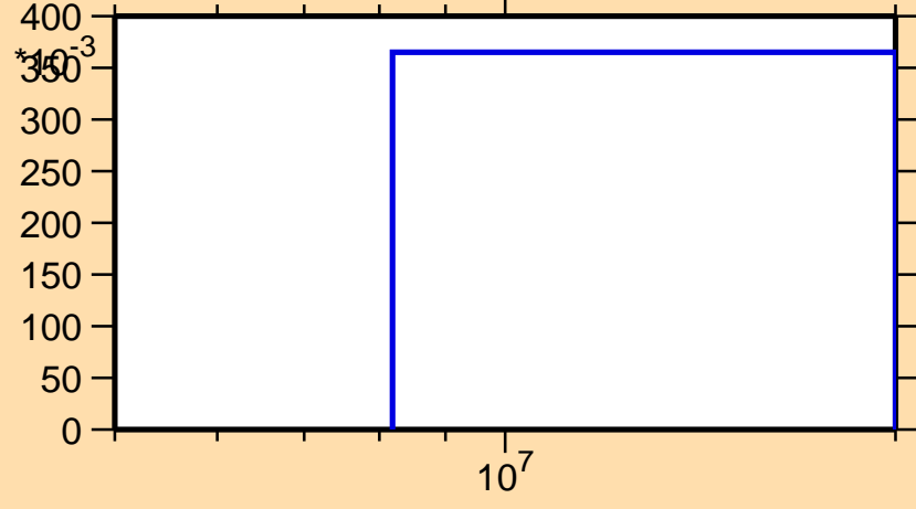
\sigma vs. E for ^{233}\text{Pa}(n,3n)
