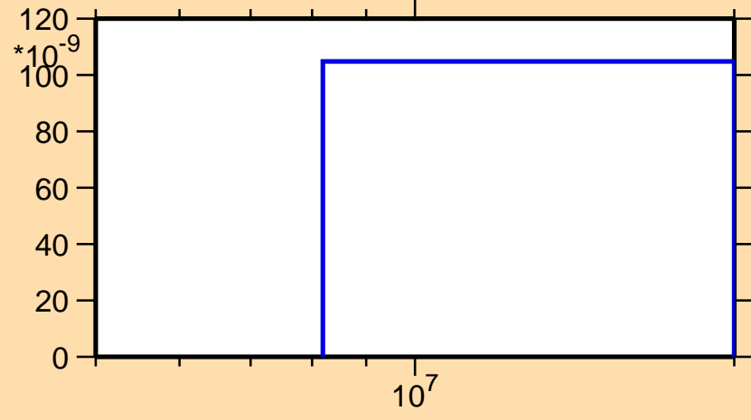
\sigma vs. E for ^{233}\text{Pa}(n,nt)
