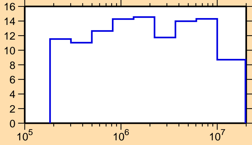
\Delta\sigma/\sigma vs. E for ^{234}\text{Pa}(n,tot.)
