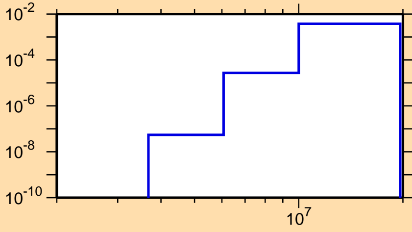
\sigma vs. E for ^{234}\text{Pa}(n,p)
