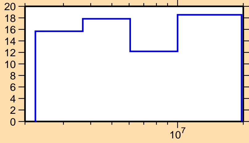
\Delta\sigma/\sigma vs. E for ^{234}\text{Pa}(n,el.)
