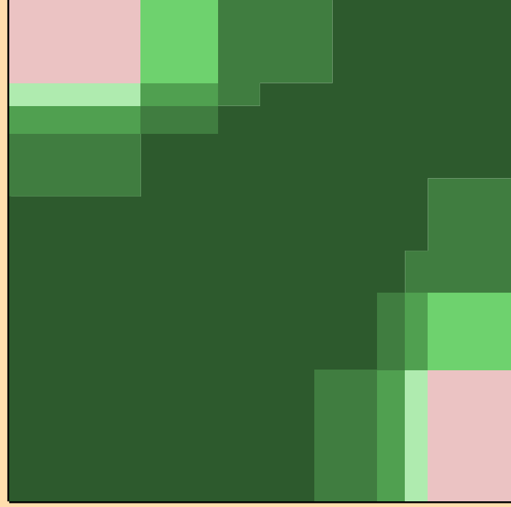
\sigma vs. E for ^{234}\text{Pa}(n,n\text{cont.})
