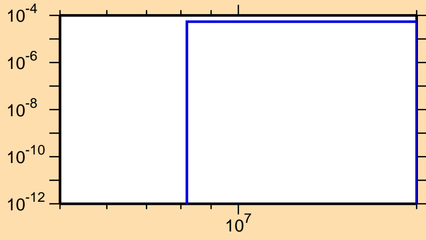
\sigma vs. E for ^{234}\text{Pa}(n,t)
