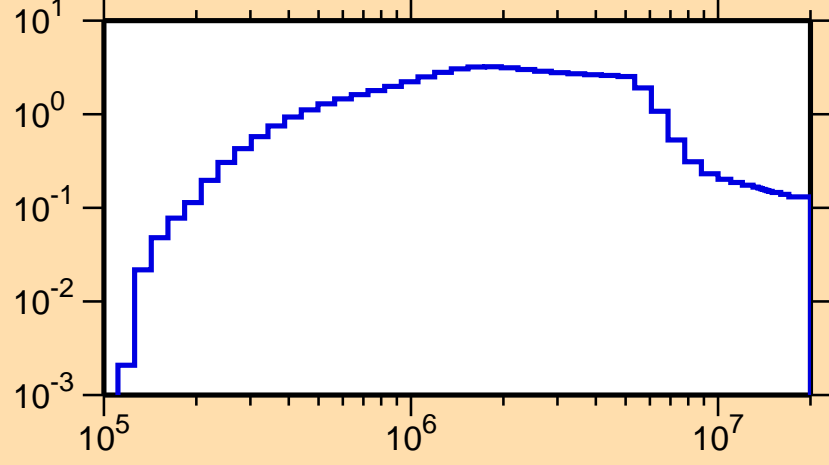
\sigma vs. E for ^{234}\text{Pa}(n,n\text{cont.})
