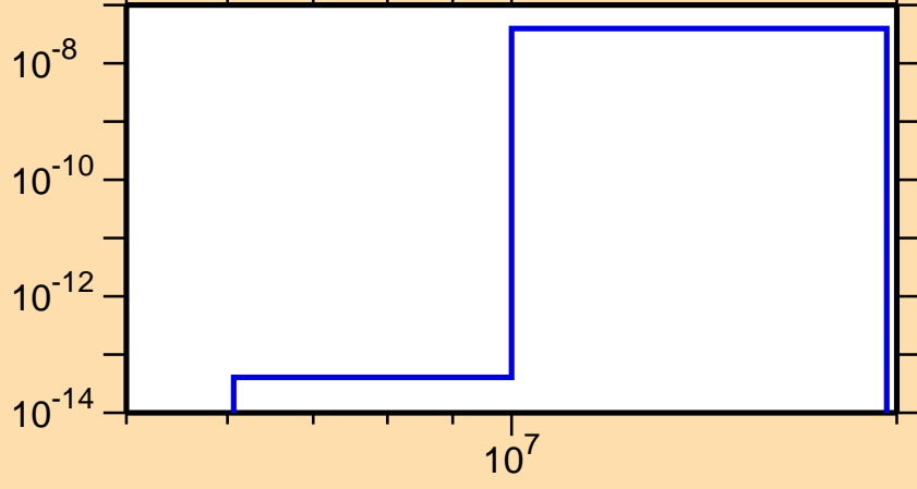
\sigma vs. E for ^{234}\text{Pa}(n,2n\alpha)
