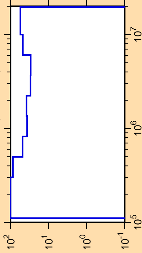
\Delta\sigma/\sigma vs. E for ^{234}\text{Pa}(n,\text{ncont.})
