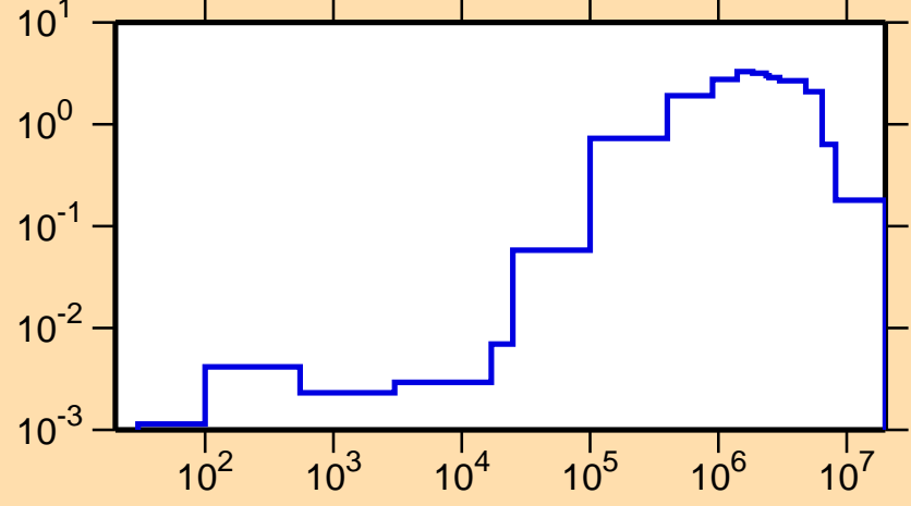
\sigma vs. E for ^{234}\text{Pa}(n,\text{inel.})
