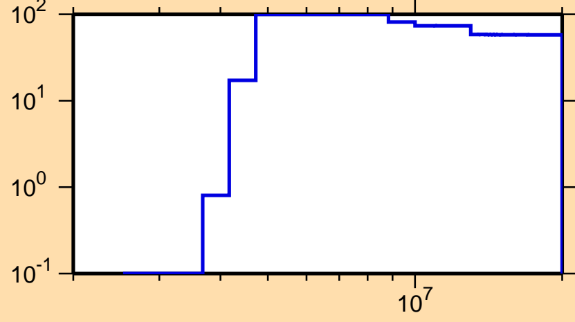
\Delta\sigma/\sigma vs. E for ^{235}\text{Pa}(n,p)
