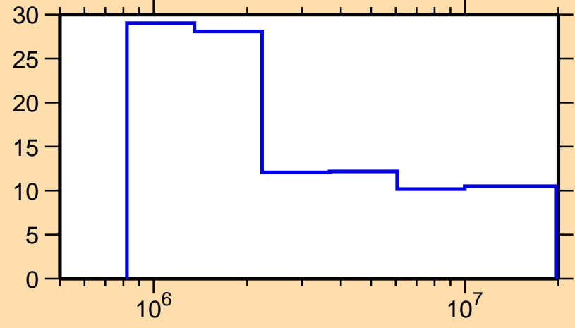
\Delta\sigma/\sigma vs. E for ^{235}\text{Pa}(n,n\text{onel.})
