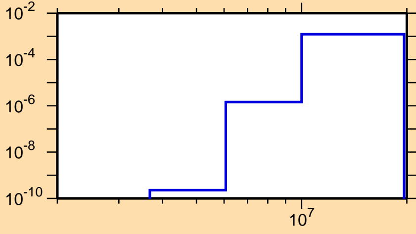
\sigma vs. E for ^{235}\text{Pa}(n,p)
