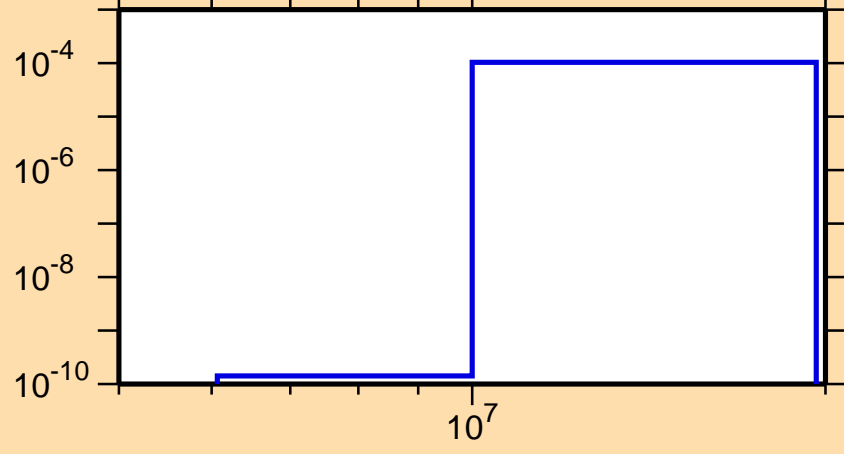
\sigma vs. E for ^{235}\text{Pa}(n,d)
