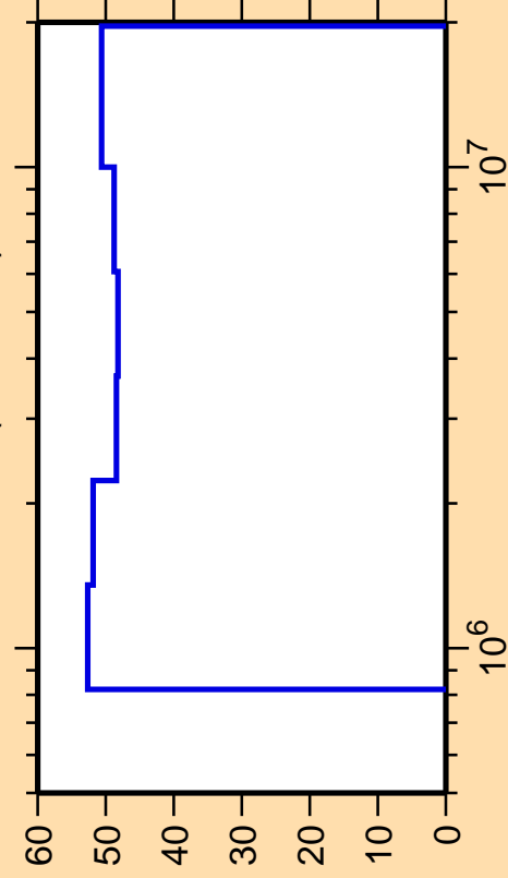
\Delta\sigma/\sigma vs. E for ^{235}\text{Pa}(n,ncont.)
