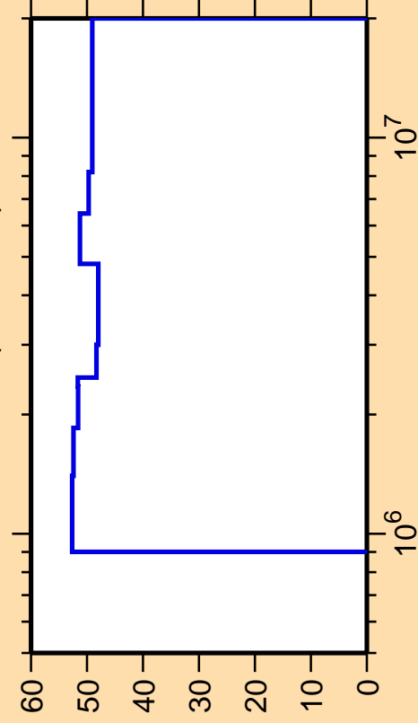
\Delta\sigma/\sigma vs. E for ^{235}\text{Pa}(n,n\text{cont.})
