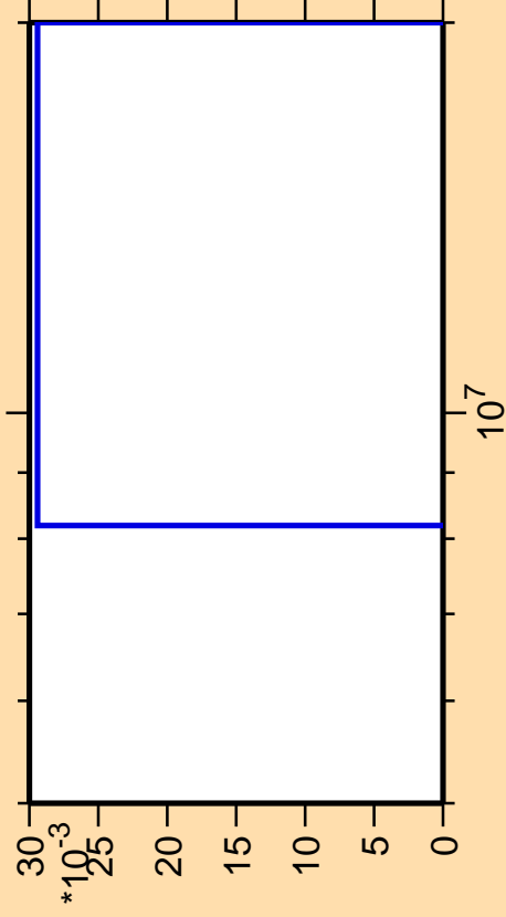
\Delta\sigma/\sigma vs. E for ^{235}\text{Pa}(\text{mt } 11)
