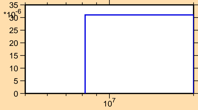
\sigma vs. E for ^{235}\text{Pa}(n,t)
