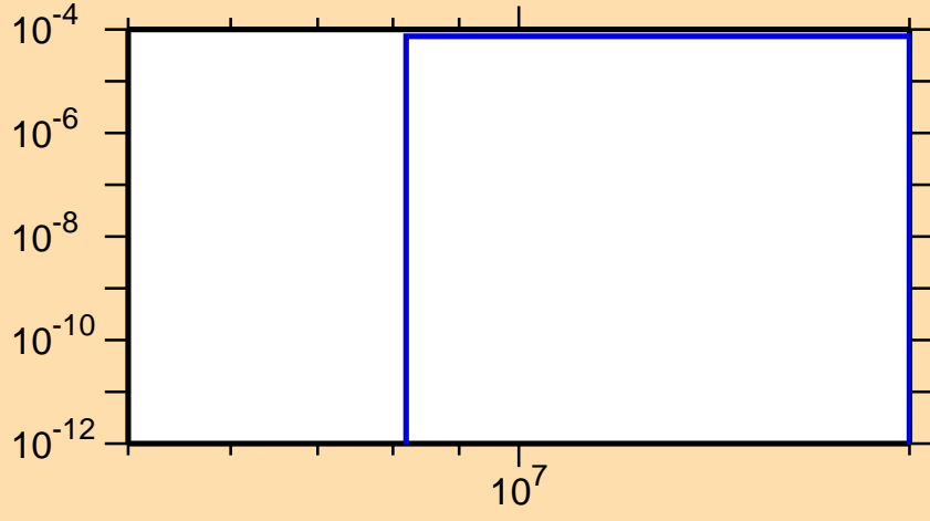
\sigma vs. E for ^{235}\text{Pa}(n,np)
