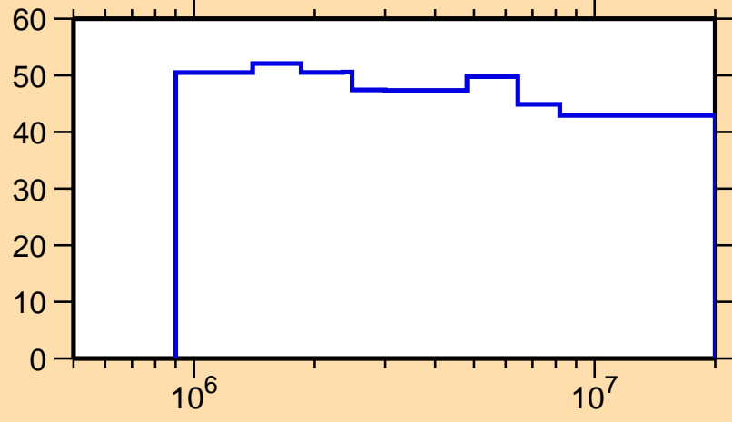
\Delta\sigma/\sigma vs. E for ^{235}\text{Pa}(n,\text{inel.})
