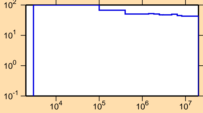
\Delta\sigma/\sigma vs. E for ^{235}\text{Pa}(n,\text{inel.})
