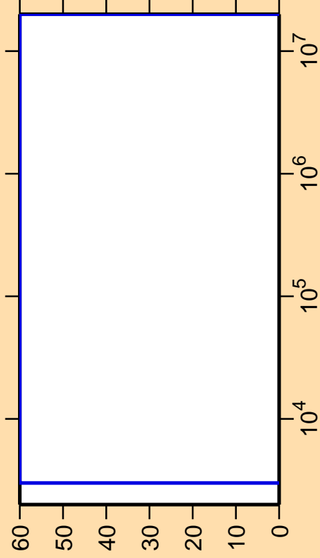
\Delta\sigma/\sigma vs. E for ^{235}\text{Pa}(n,f)
