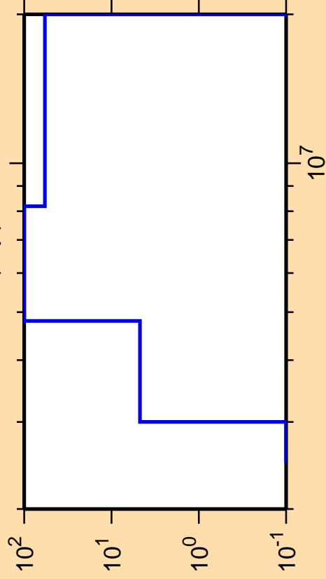
\Delta\sigma/\sigma vs. E for ^{235}\text{Pa}(n,p)
