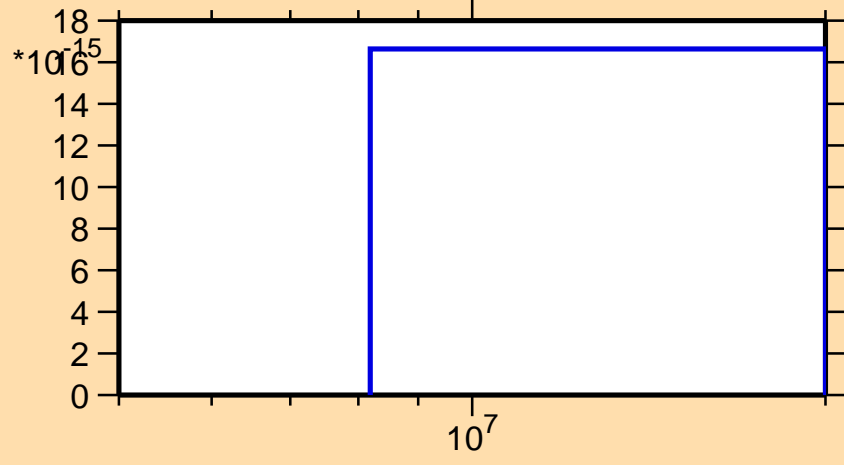
\sigma vs. E for ^{235}\text{Pa}(\text{mt } 11)
