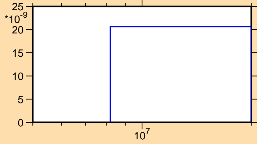
\sigma vs. E for ^{235}\text{Pa}(n,\text{nd})
