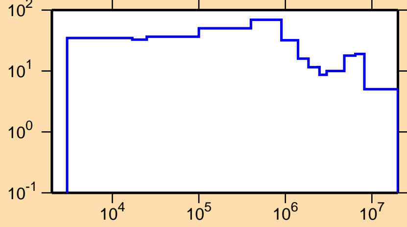
\Delta\sigma/\sigma vs. E for ^{235}\text{Pa}(n,\text{el.})
