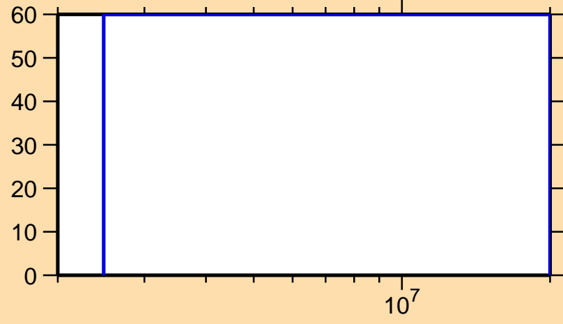
\Delta\sigma/\sigma vs. E for ^{235}\text{Pa}(n,n_1)
