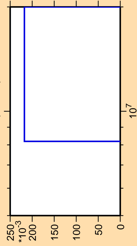
\Delta\sigma/\sigma vs. E for ^{235}\text{Pa}(n,3n\alpha)
