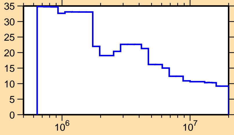
\Delta\sigma/\sigma vs. E for ^{236}\text{Pa}(n,n\text{nonel.})
