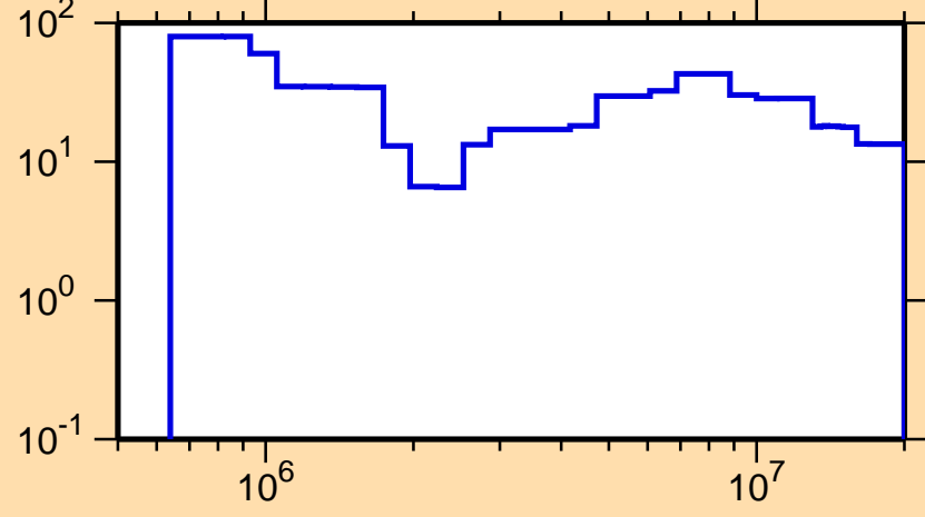
\Delta\sigma/\sigma vs. E for ^{236}\text{Pa}(n,\text{el.})
