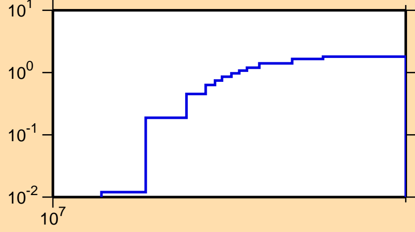
\sigma vs. E for ^{236}\text{Pa}(n,3n)
