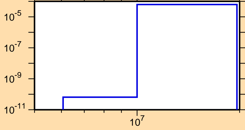
\sigma vs. E for ^{236}\text{Pa}(n,t)
