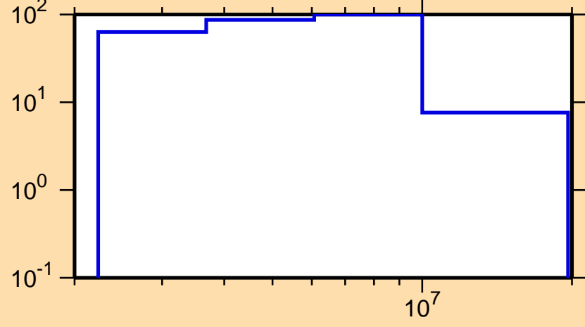
\Delta\sigma/\sigma vs. E for ^{236}\text{Pa}(n,n_1)
