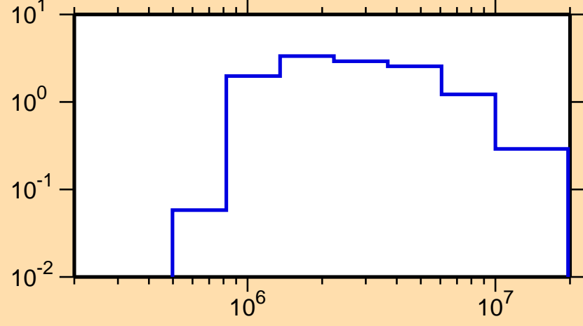
\sigma vs. E for ^{236}\text{Pa}(n,n\text{cont.})
