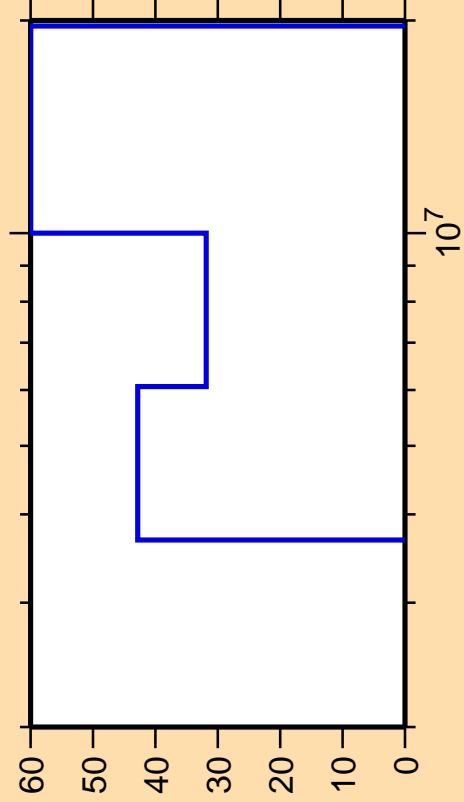
\Delta\sigma/\sigma vs. E for ^{236}\text{Pa}(n,\gamma)
