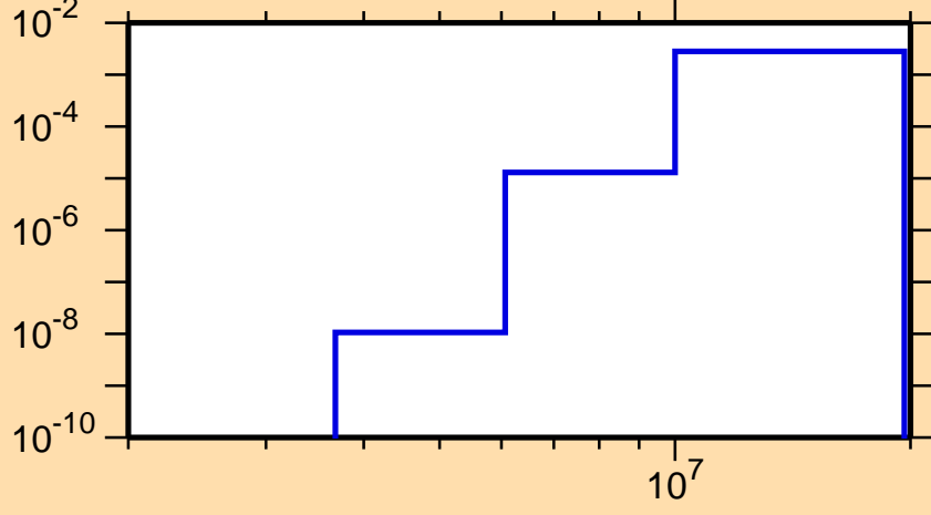
\sigma vs. E for ^{236}\text{Pa}(n,p)
