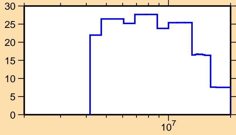
\Delta\sigma/\sigma vs. E for ^{237}\text{Pa}(n,el.)
