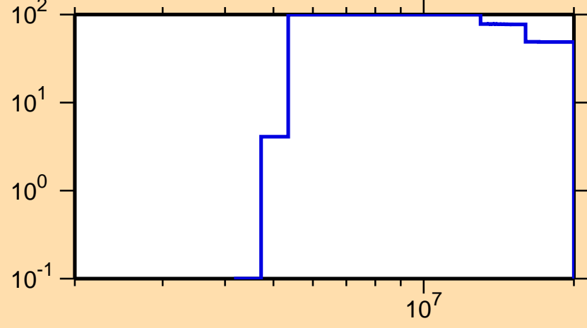
\Delta\sigma/\sigma vs. E for ^{237}\text{Pa}(n,p)
