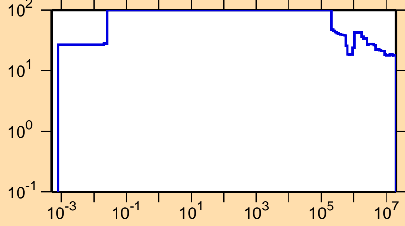
\Delta\sigma/\sigma vs. E for ^{237}\text{Pa}(n,\text{nonel.})
