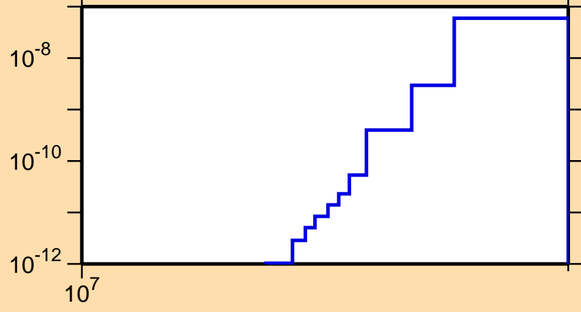
\sigma vs. E for ^{237}\text{Pa}(n,2n\alpha)
