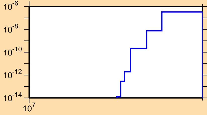
\sigma vs. E for ^{237}\text{Pa}(n,2np)
