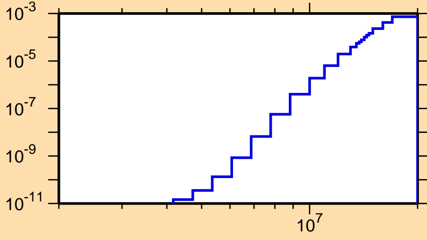
\sigma vs. E for ^{237}\text{Pa}(n,\alpha)
