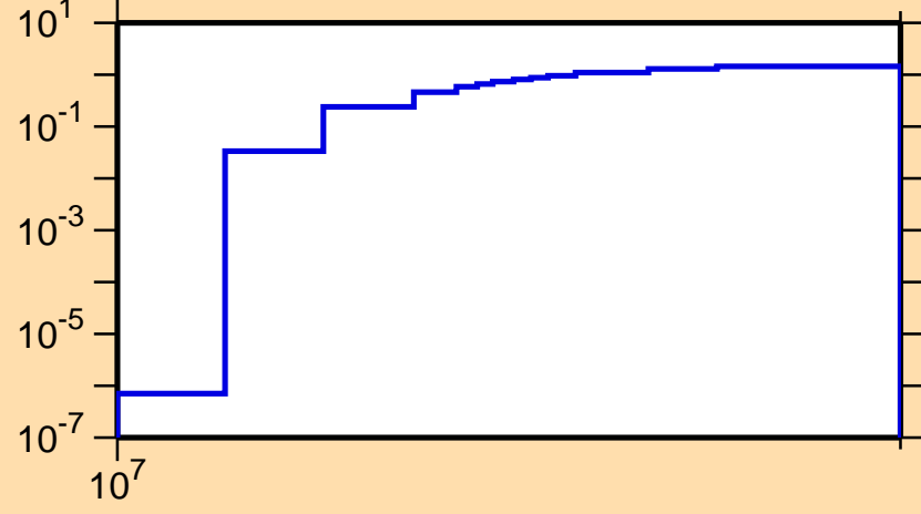
\sigma vs. E for ^{237}\text{Pa}(n,3n)
