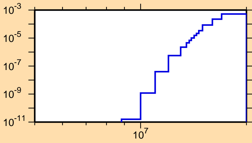
\sigma vs. E for ^{237}\text{Pa}(n,t)
