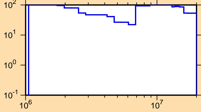
\Delta\sigma/\sigma vs. E for ^{237}\text{Pa}(n,n\text{cont.})
