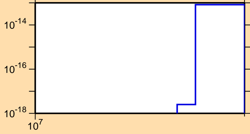
\sigma vs. E for ^{237}\text{Pa}(n,\text{He3})
