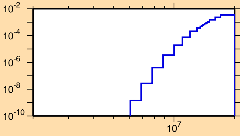
\sigma vs. E for ^{237}\text{Pa}(n,p)
