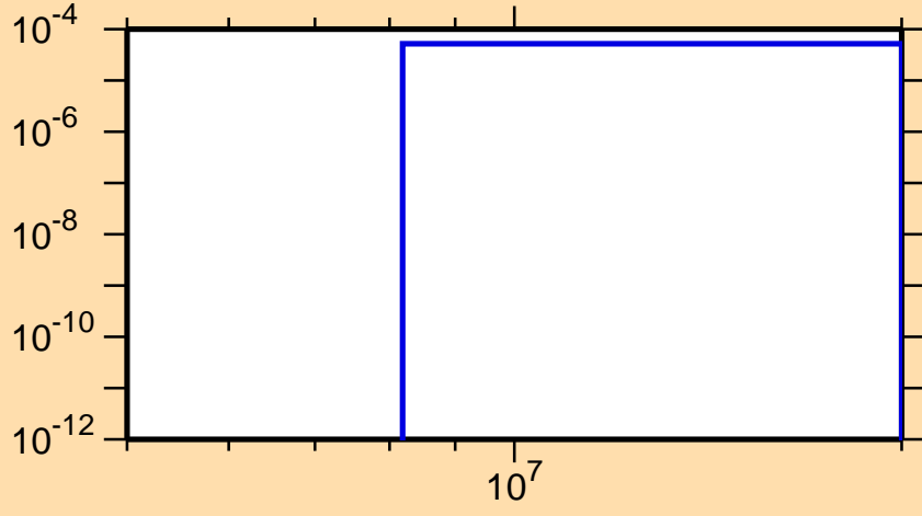
\sigma vs. E for ^{237}\text{Pa}(n,d)
