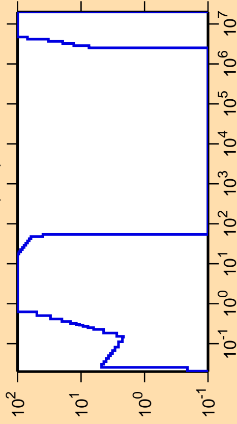
\Delta\sigma/\sigma vs. E for ^{238}\text{Pa}(n,\alpha)
