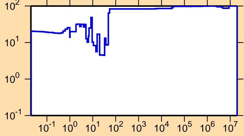
\Delta\sigma/\sigma vs. E for ^{238}\text{Pa}(n,\gamma)
