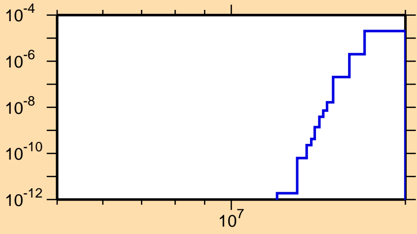
\sigma vs. E for ^{238}\text{Pa}(n,\text{nt})
