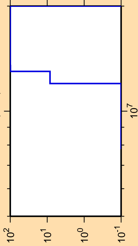
\Delta\sigma/\sigma vs. E for ^{238}\text{Pa}(n,\text{nt})
