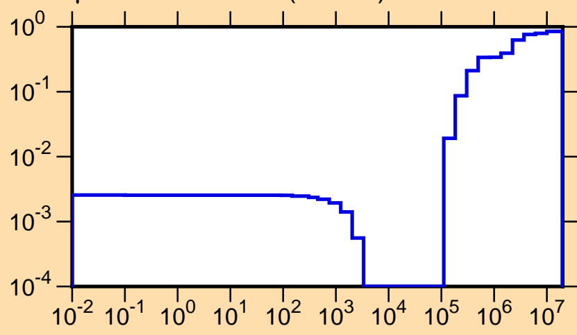
\mu vs. E for ^{238}\text{Pa}(\text{mt251})
