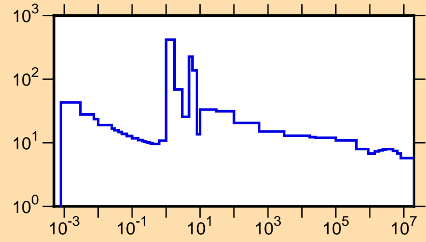
\sigma vs. E for ^{238}\text{Pa}(n,\text{tot.})
