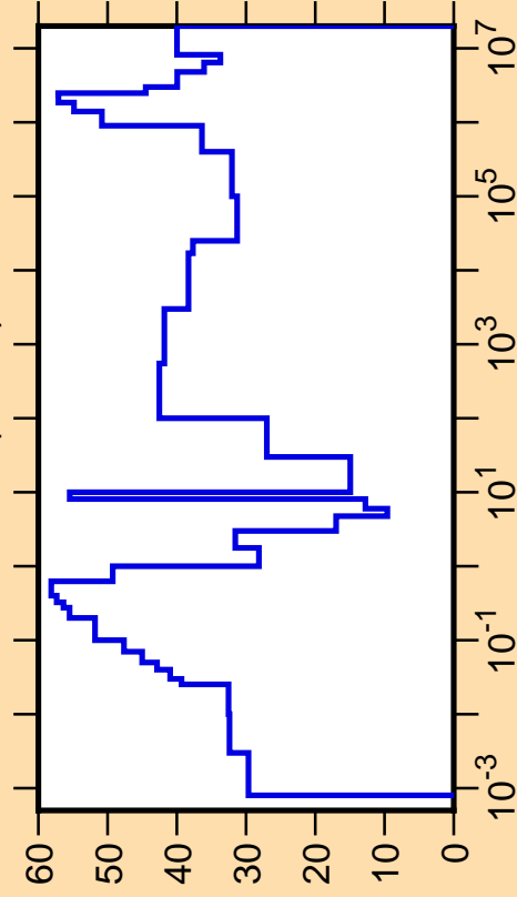
\Delta\sigma/\sigma vs. E for ^{238}\text{Pa}(n,\text{tot.})
