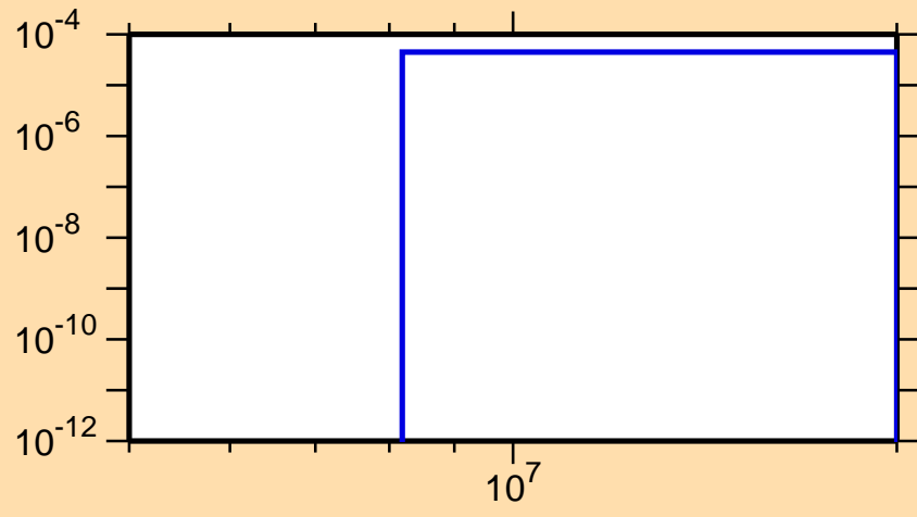
\sigma vs. E for ^{238}\text{Pa}(n,t)
