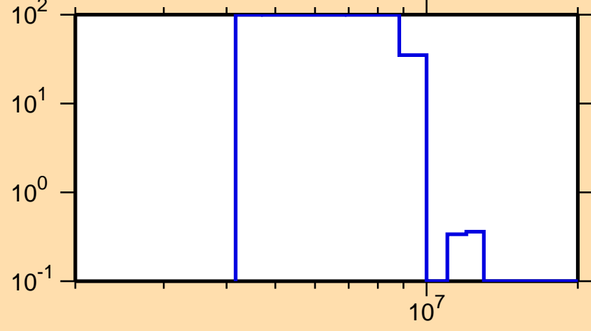
\Delta\sigma/\sigma vs. E for ^{239}\text{Pa}(n,n_1)
