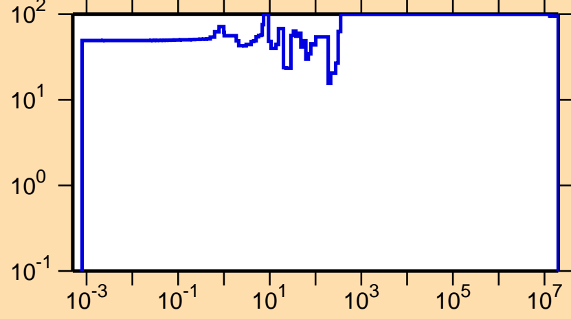
\Delta\sigma/\sigma vs. E for ^{239}\text{Pa}(n,f)
