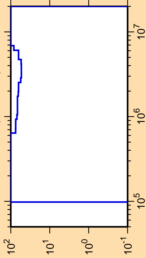
\Delta\sigma/\sigma vs. E for ^{239}\text{Pa}(n,\text{ncont.})
