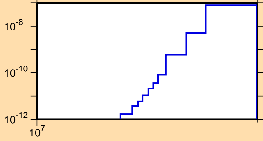
\sigma vs. E for ^{239}\text{Pa}(n,2n\alpha)
