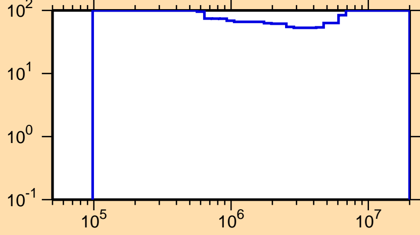
\Delta\sigma/\sigma vs. E for ^{239}\text{Pa}(n,\text{inel.})
