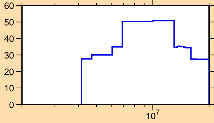
\Delta\sigma/\sigma vs. E for ^{239}\text{Pa}(n,el.)
