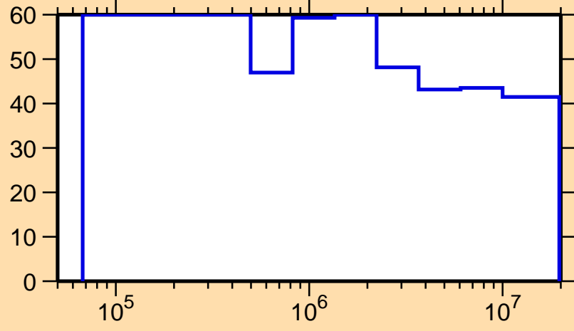
\Delta\sigma/\sigma vs. E for ^{239}\text{Pa}(n,n\text{nonel.})
