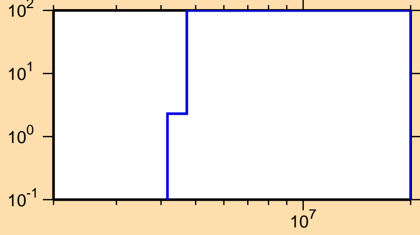
\Delta\sigma/\sigma vs. E for ^{240}\text{Pa}(n,p)
