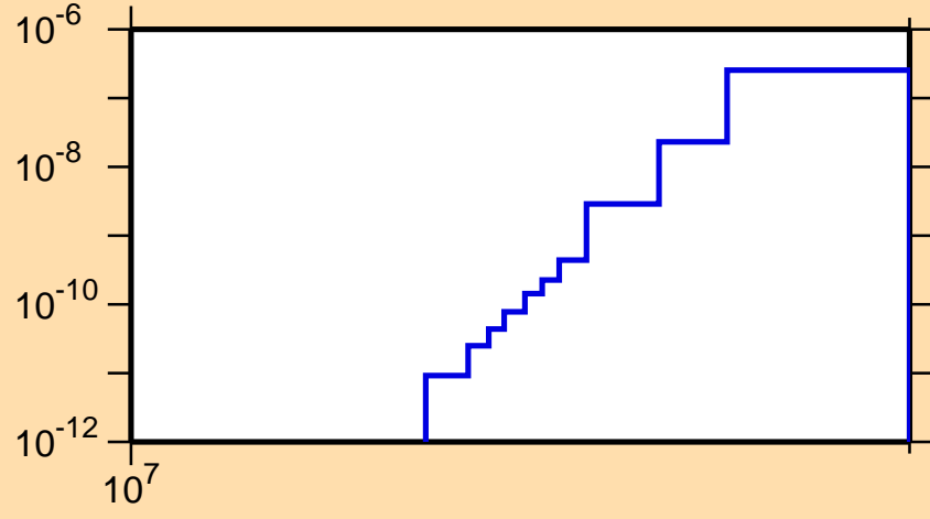
\sigma vs. E for ^{240}\text{Pa}(n,2n\alpha)
