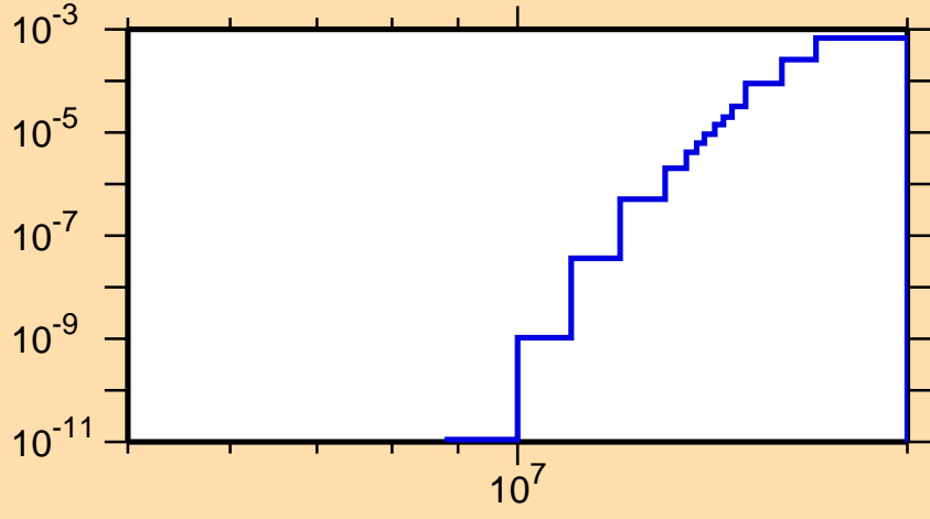
\sigma vs. E for ^{240}\text{Pa}(n,d)
