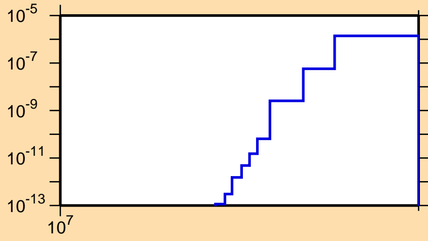
\sigma vs. E for ^{240}\text{Pa}(n,2np)
