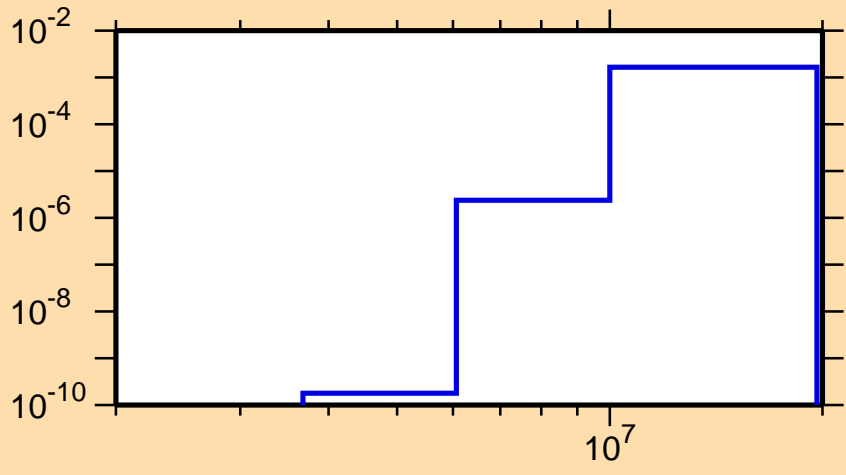
\sigma vs. E for ^{240}\text{Pa}(n,p)
