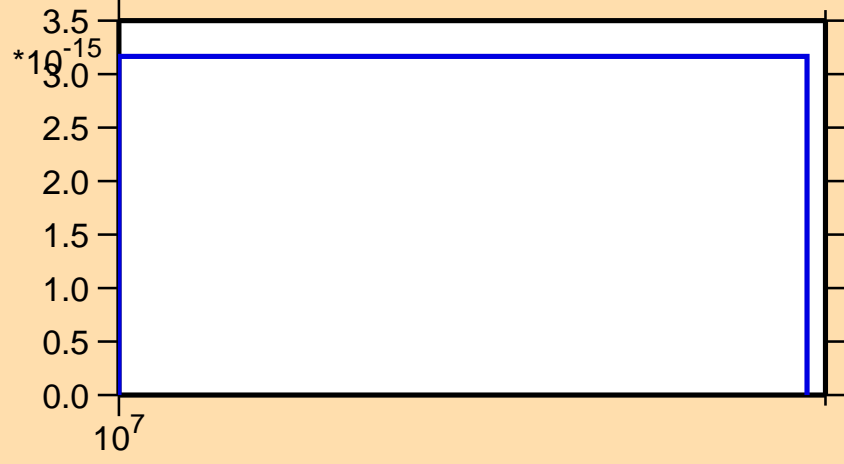
\sigma vs. E for ^{240}\text{Pa} (mt 42)
