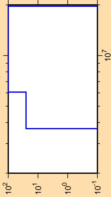
\Delta\sigma/\sigma vs. E for ^{240}\text{Pa}(n,\alpha)
