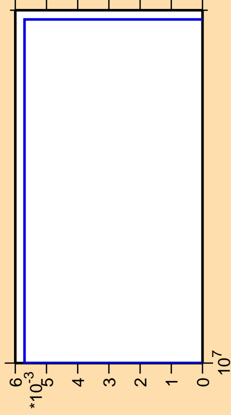
\Delta\sigma/\sigma vs. E for ^{240}\text{Pa}(n,\text{He3})
