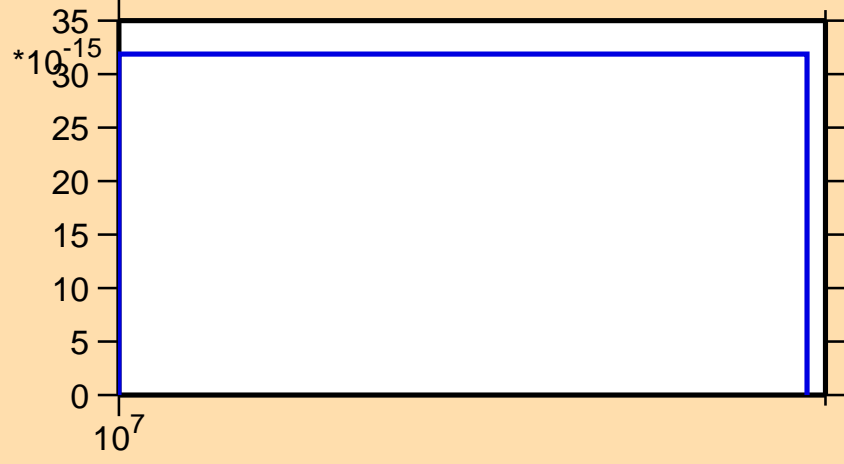
\sigma vs. E for ^{240}\text{Pa}(n,3n\alpha)
