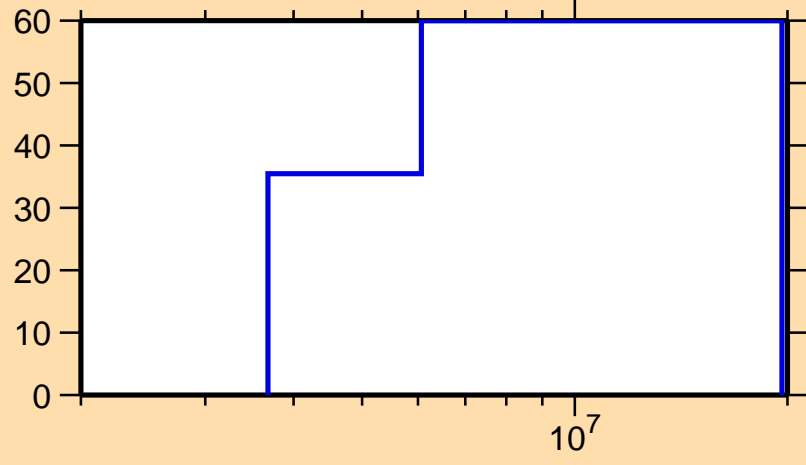
\Delta\sigma/\sigma vs. E for ^{240}\text{Pa}(n,el.)
