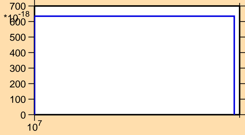
\sigma vs. E for ^{240}\text{Pa}(n,\text{He3})
