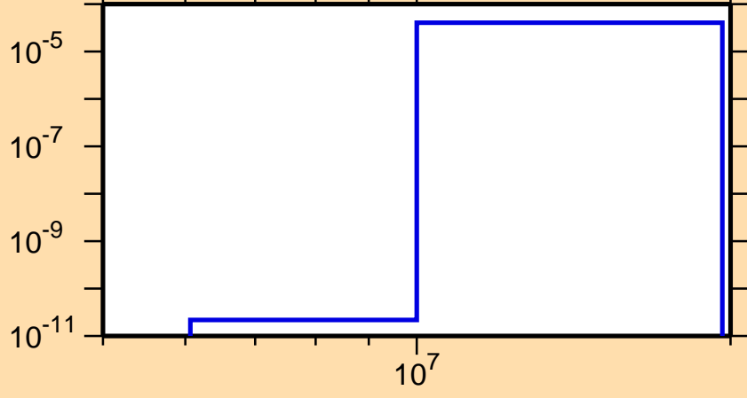
\sigma vs. E for ^{240}\text{Pa}(n,t)
