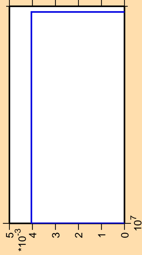
\Delta\sigma/\sigma vs. E for ^{240}\text{Pa} (mt 42)
