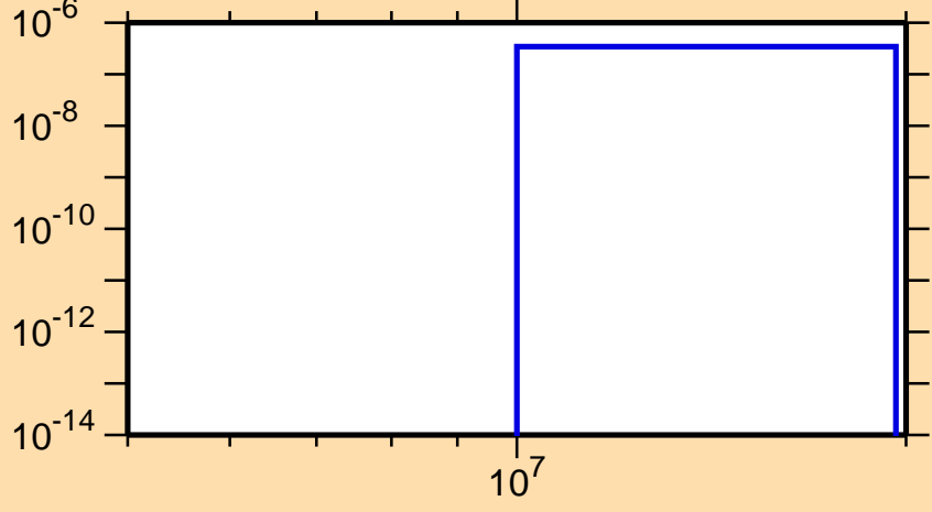
\sigma vs. E for ^{240}\text{Pa}(n,nt)
