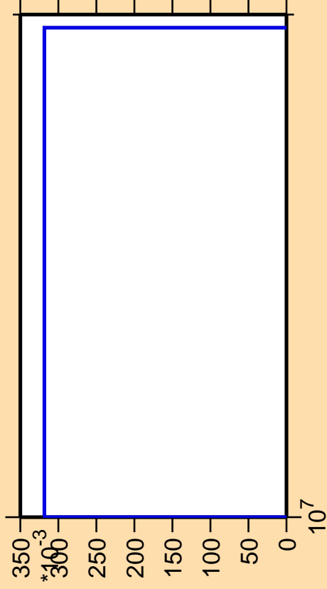
\Delta\sigma/\sigma vs. E for ^{240}\text{Pa} (mt 11)
