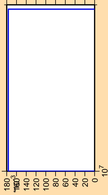
\Delta\sigma/\sigma vs. E for ^{240}\text{Pa}(n,3n\alpha)
