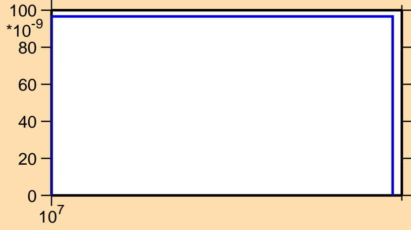
\sigma vs. E for ^{240}\text{Pa}(n,\text{nd})
