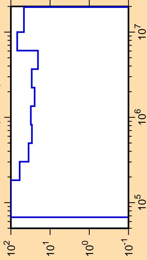
\Delta\sigma/\sigma vs. E for ^{240}\text{Pa}(n,\text{inel.})
