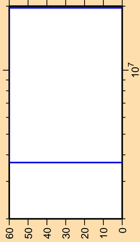
\Delta\sigma/\sigma vs. E for ^{240}\text{Pa}(n,\gamma)
