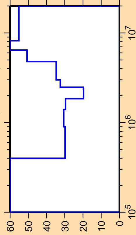
\Delta\sigma/\sigma vs. E for ^{240}\text{Pa}(n,n\text{cont.})
