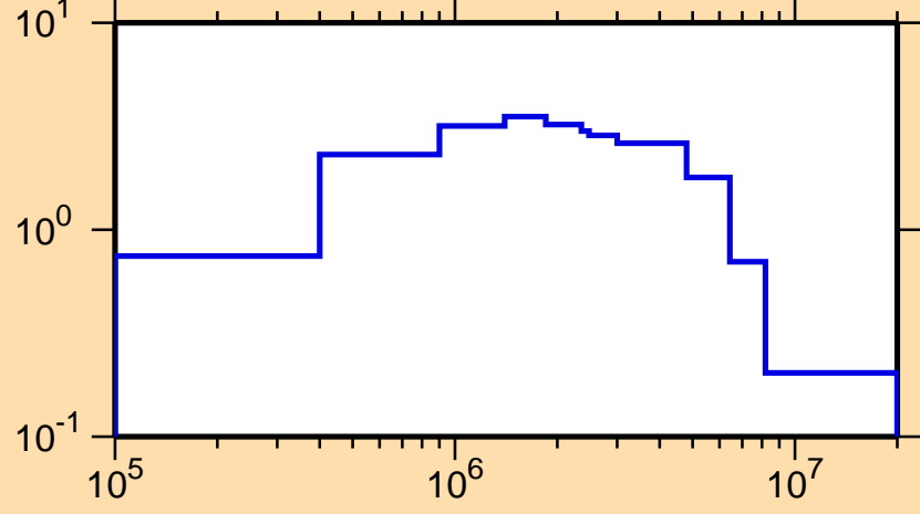
\sigma vs. E for ^{240}\text{Pa}(n,n\text{cont.})
