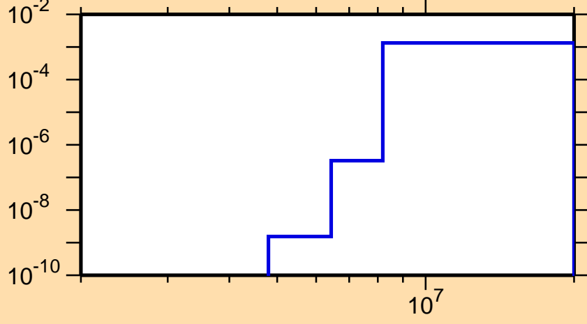
\sigma vs. E for ^{240}\text{Pa}(n,p)
