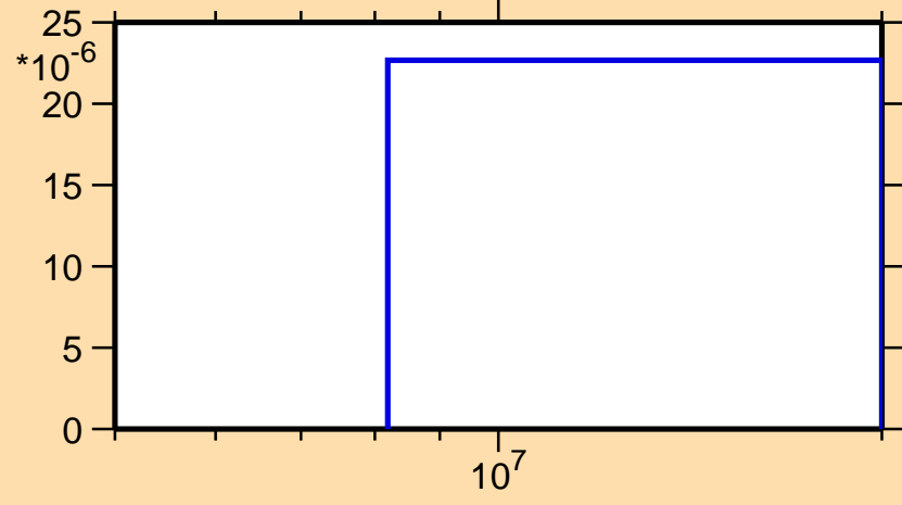
\sigma vs. E for ^{240}\text{Pa}(n,np)
