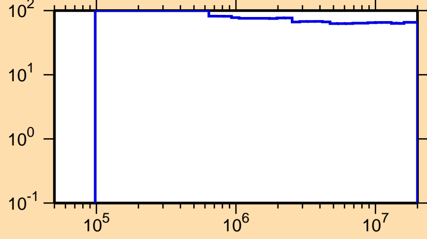
\Delta\sigma/\sigma vs. E for ^{241}\text{Pa}(n,n_1)
