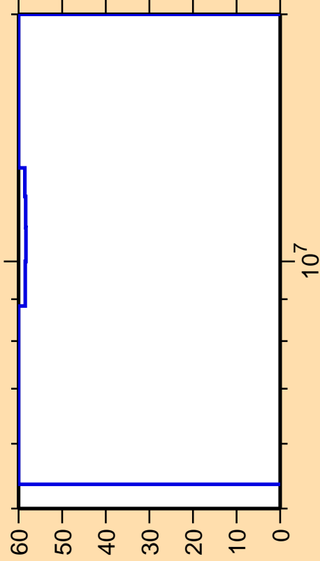
\Delta\sigma/\sigma vs. E for ^{241}\text{Pa}(n,2n)
