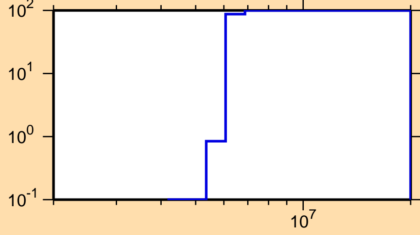
\Delta\sigma/\sigma vs. E for ^{241}\text{Pa}(n,p)
