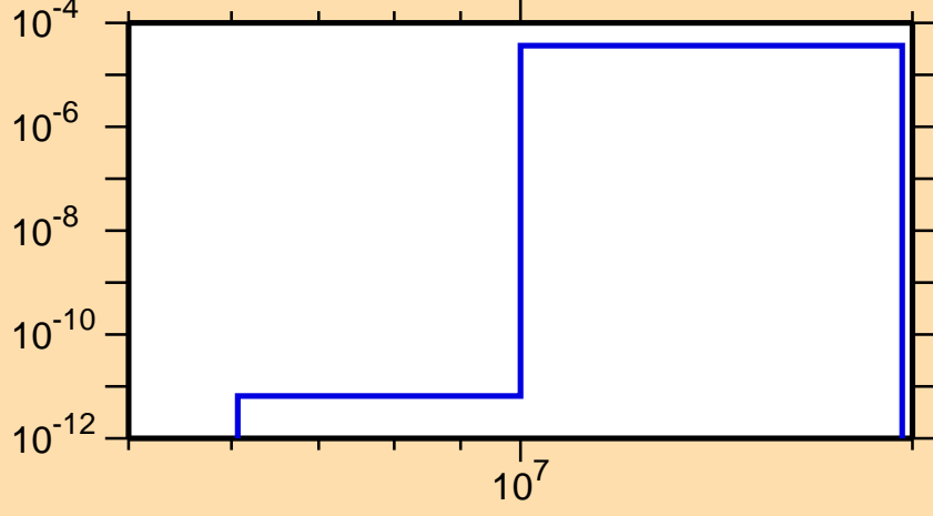
\sigma vs. E for ^{241}\text{Pa}(n,d)
