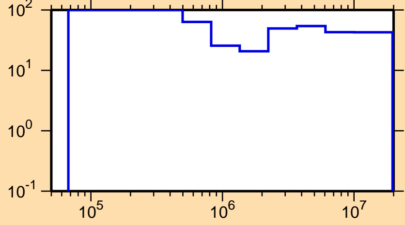
\Delta\sigma/\sigma vs. E for ^{241}\text{Pa}(n,\text{nonel.})
