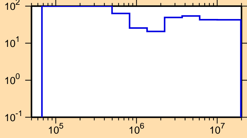
\Delta\sigma/\sigma vs. E for ^{241}\text{Pa}(n,n\text{onel.})
