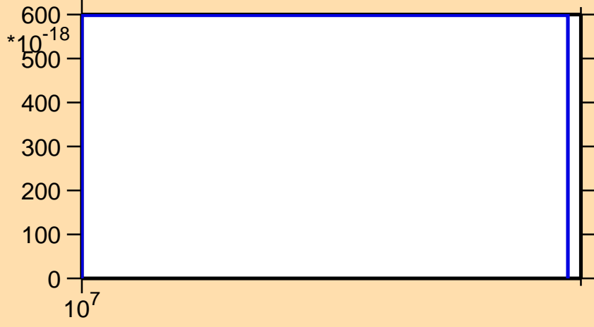
\sigma vs. E for ^{241}\text{Pa} (mt 42)
