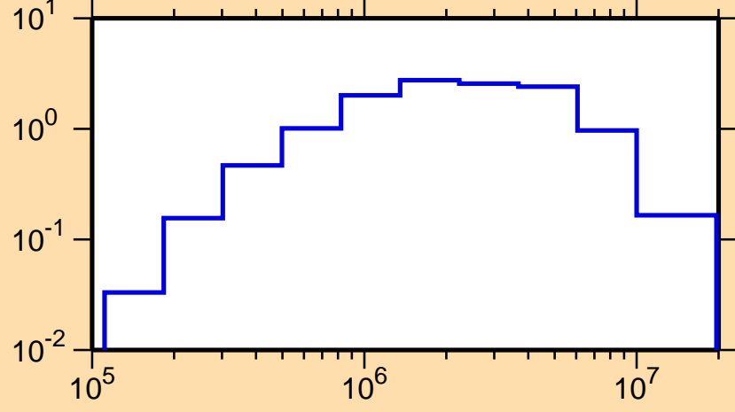
\sigma vs. E for ^{241}\text{Pa}(n,n\text{cont.})
