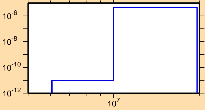
\sigma vs. E for ^{241}\text{Pa}(n,n\alpha)
