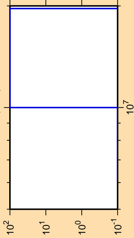
\Delta\sigma/\sigma vs. E for ^{241}\text{Pa}(n,\text{nt})
