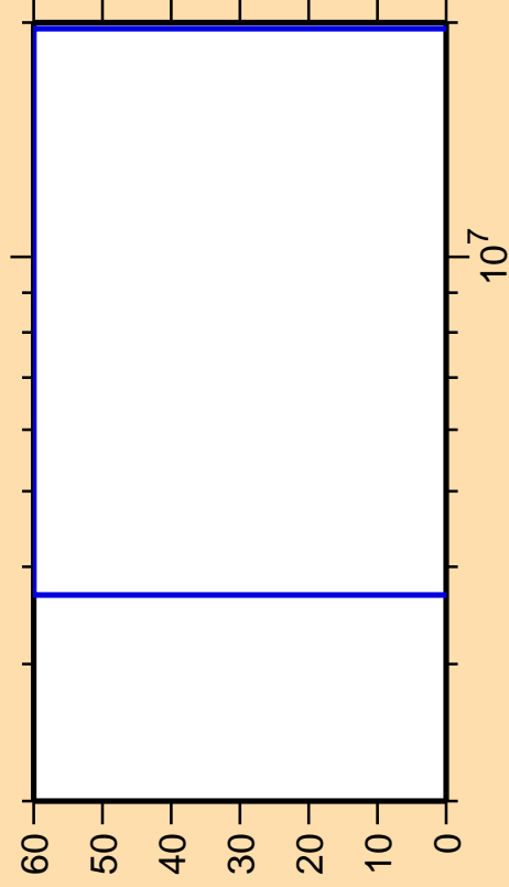
\Delta\sigma/\sigma vs. E for ^{241}\text{Pa}(n,f)
