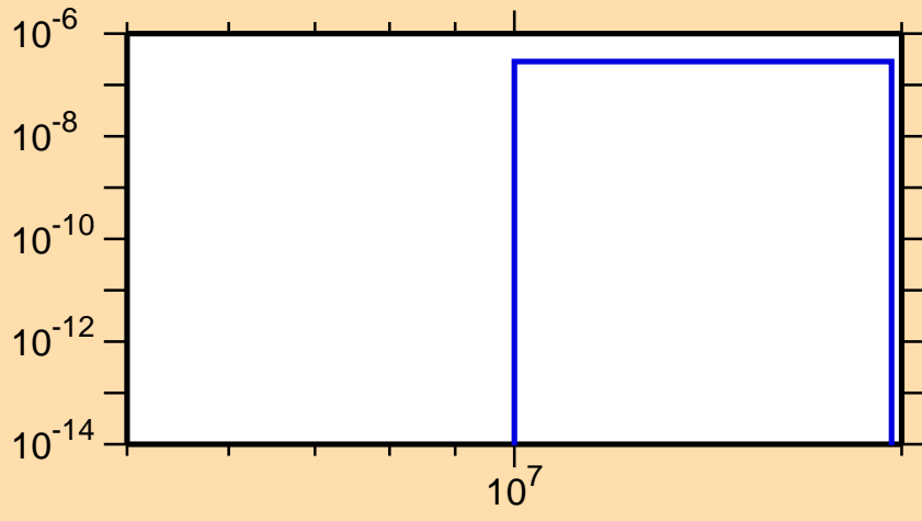
\sigma vs. E for ^{241}\text{Pa}(n,\text{nt})
