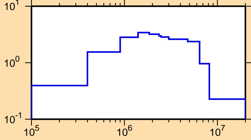
\sigma vs. E for ^{241}\text{Pa}(n,\text{inel.})
