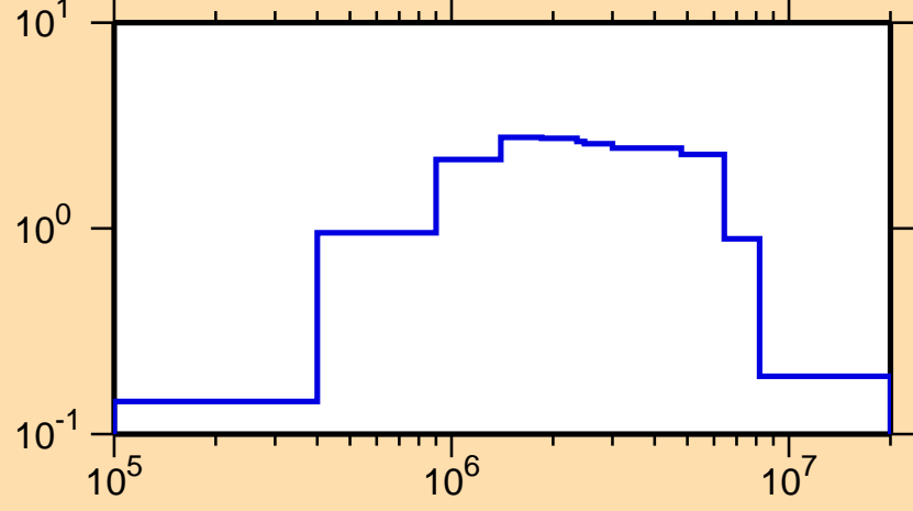
\sigma vs. E for ^{241}\text{Pa}(n,n\text{cont.})
