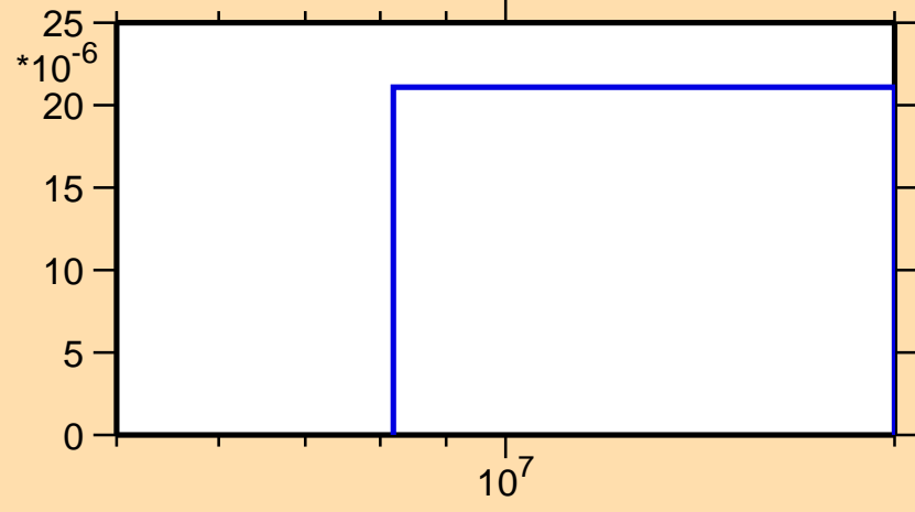
\sigma vs. E for ^{241}\text{Pa}(n,np)
