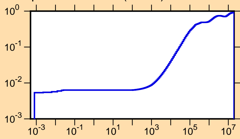
\mu vs. E for ^{127}\text{Pm}(\text{mt251})
