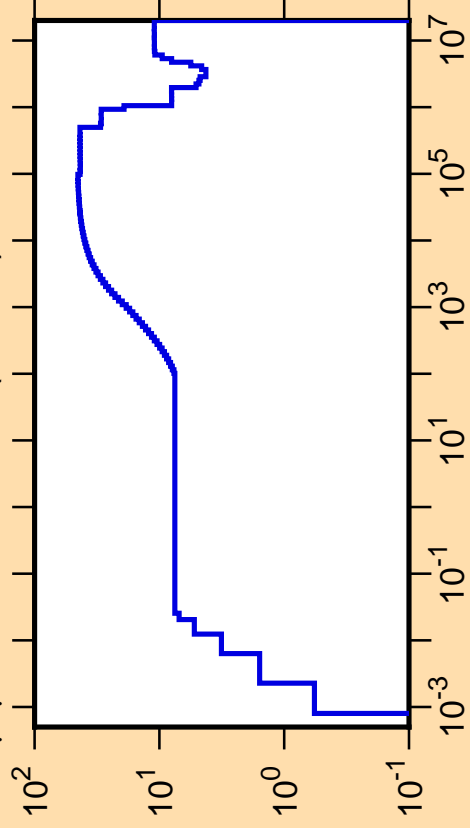
\Delta\mu/\mu vs. E for ^{127}\text{Pm}(\text{mt251})
