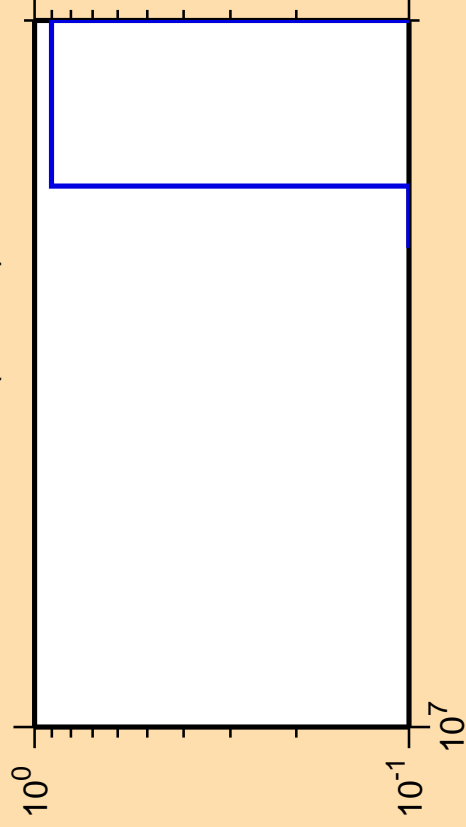
\Delta\sigma/\sigma vs. E for ^{127}\text{Pm}(n,2n\alpha)
