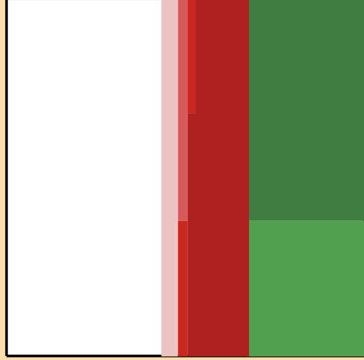
\Delta\sigma/\sigma vs. E for ^{127}\text{Pm}(n,2n)
