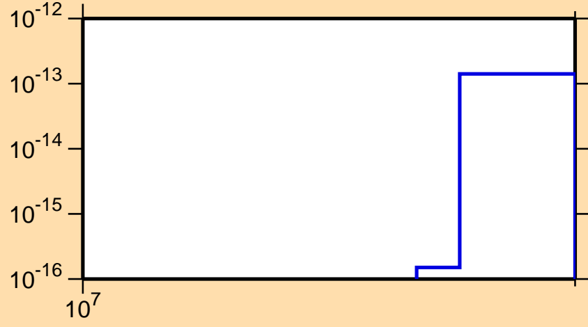
\sigma vs. E for ^{127}\text{Pm}(n,2n\alpha)
