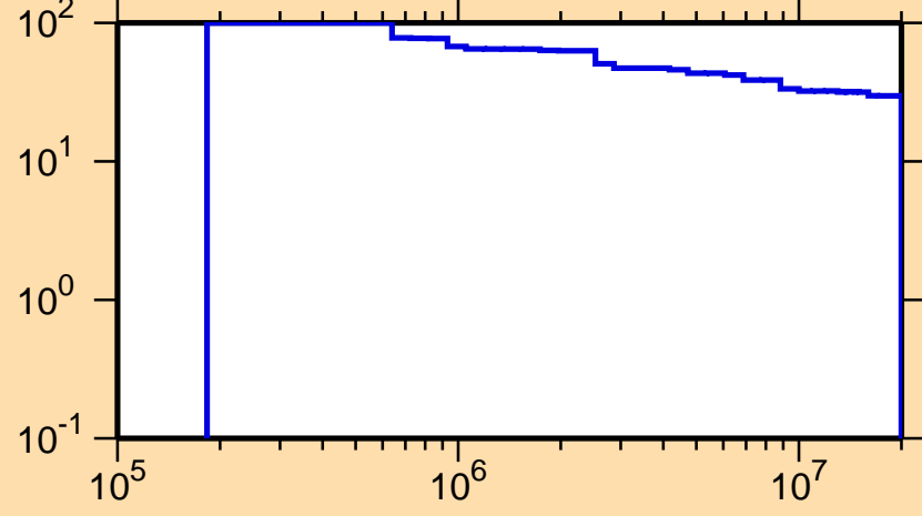
\Delta\sigma/\sigma vs. E for ^{127}\text{Pm}(n,\text{inel.})
