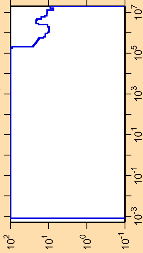
\Delta\sigma/\sigma vs. E for ^{127}\text{Pm}(n,\text{el.})
