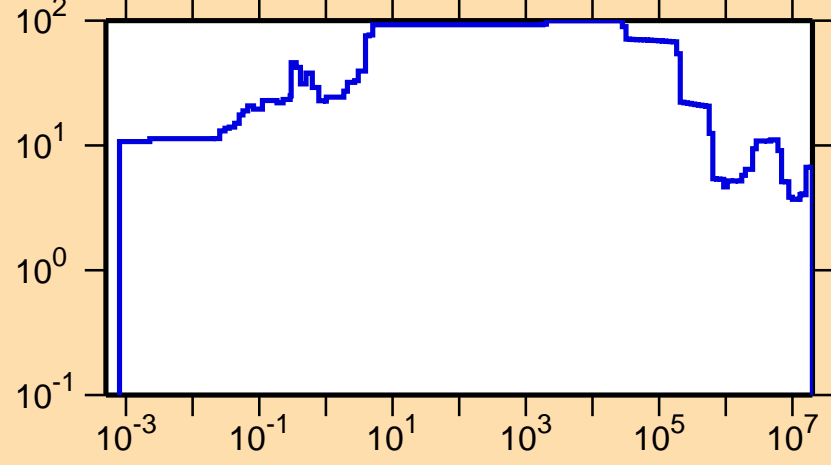
\Delta\sigma/\sigma vs. E for ^{127}\text{Pm}(n,\text{tot.})
