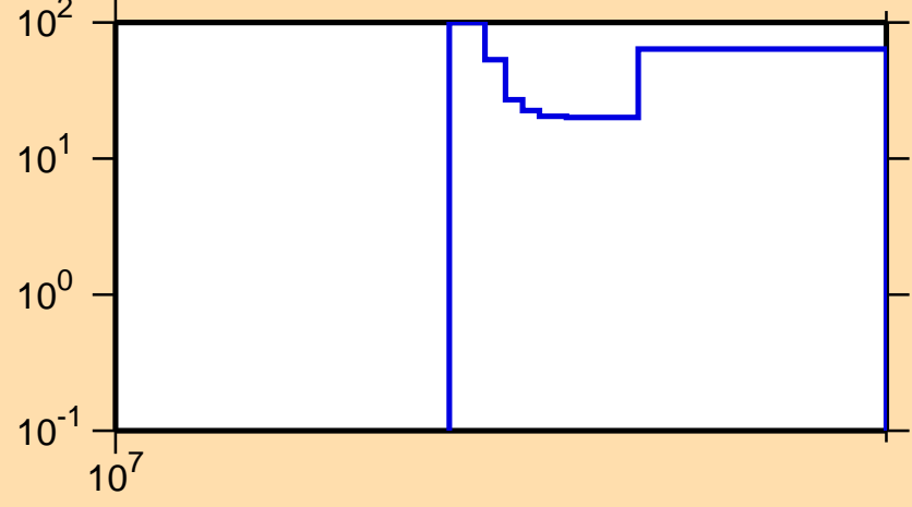
\Delta\sigma/\sigma vs. E for ^{127}\text{Pm}(n,2n)
