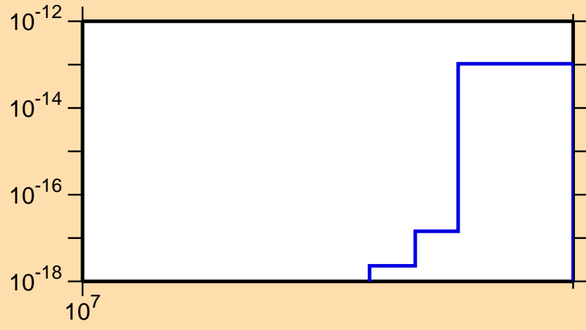
\sigma vs. E for ^{127}\text{Pm}(n,nt)
