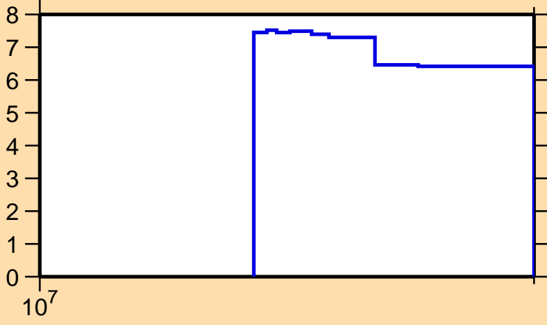
\Delta\sigma/\sigma vs. E for ^{127}\text{Pm}(n,\text{nonel.})
