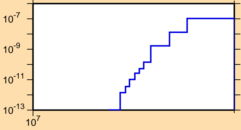
\sigma vs. E for ^{127}\text{Pm}(n,nd)
