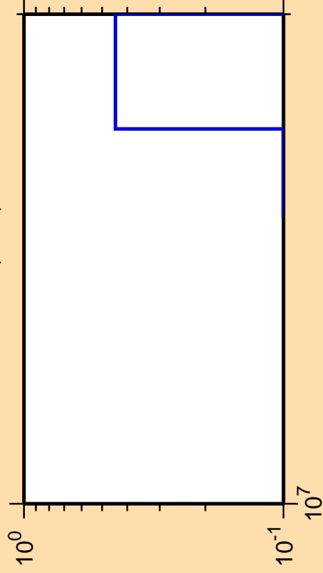
\Delta\sigma/\sigma vs. E for ^{127}\text{Pm}(n,nt)
