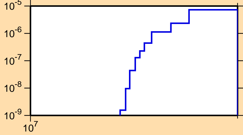
\sigma vs. E for ^{127}\text{Pm}(n,2n)
