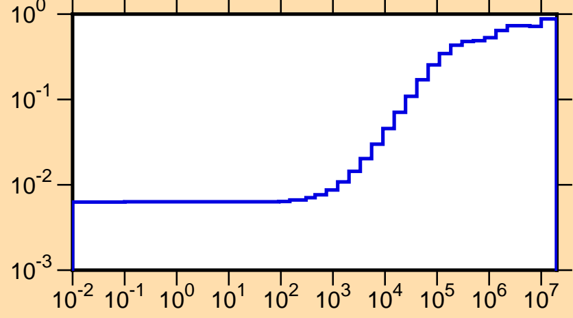
\mu vs. E for ^{127}\text{Pm}(\text{mt251})
