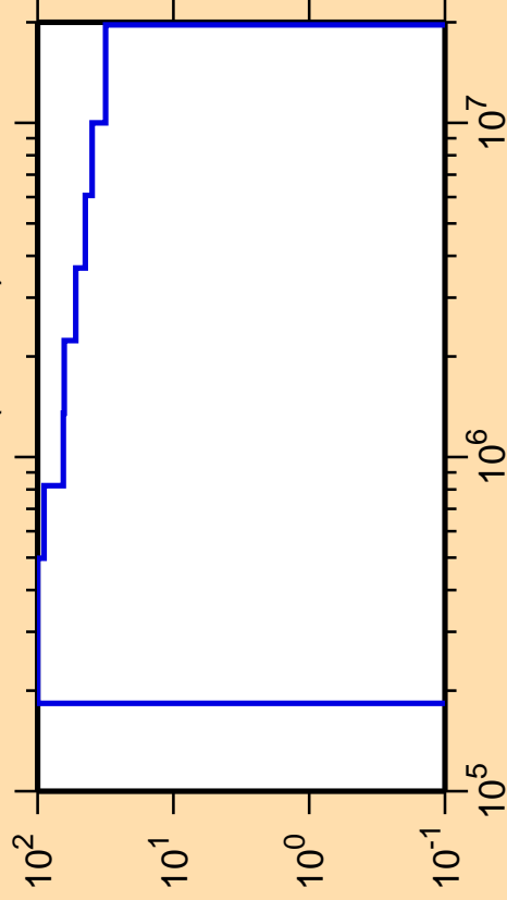
\Delta\sigma/\sigma vs. E for ^{127}\text{Pm}(n,\text{inel.})
