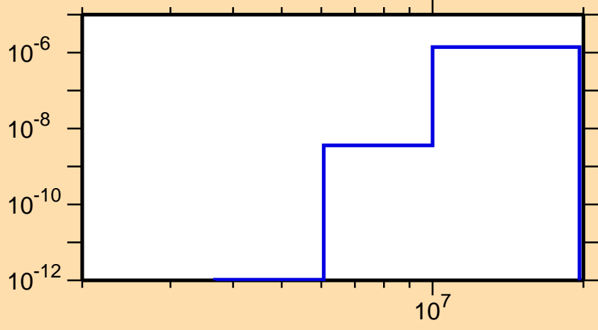
\sigma vs. E for ^{127}\text{Pm}(\text{mt117})
