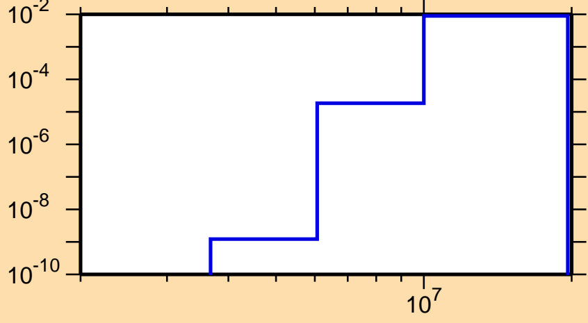
\sigma vs. E for ^{127}\text{Pm}(n,\text{pd})
