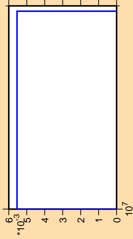
\Delta\sigma/\sigma vs. E for ^{127}\text{Pm}(n,2n\alpha)
