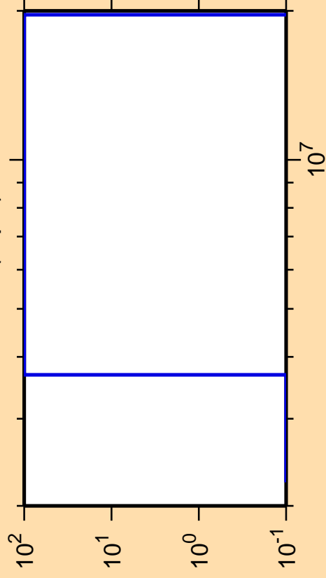
\Delta\sigma/\sigma vs. E for ^{127}\text{Pm}(n,\text{pd})
