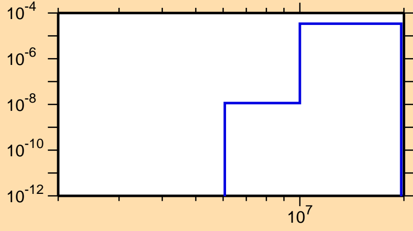
\sigma vs. E for ^{127}\text{Pm} (mt 45)
