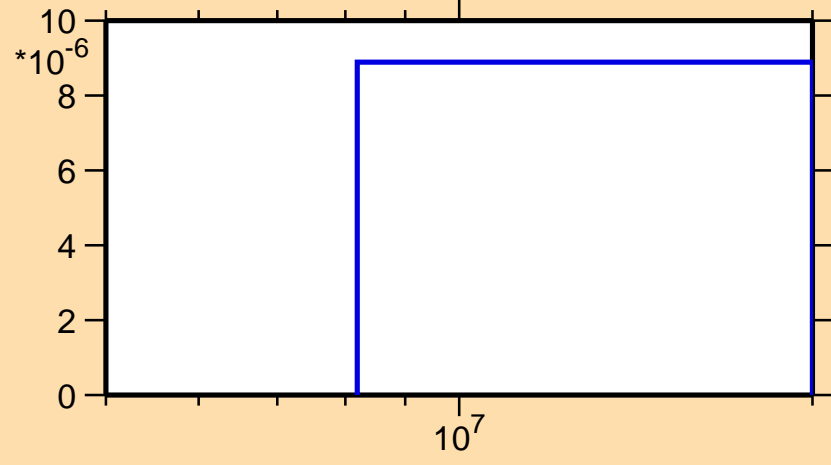
\sigma vs. E for ^{127}\text{Pm}(n,pt)
