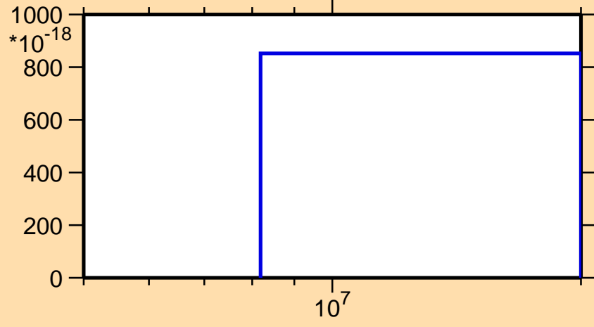
\sigma vs. E for ^{127}\text{Pm}(n,nt)
