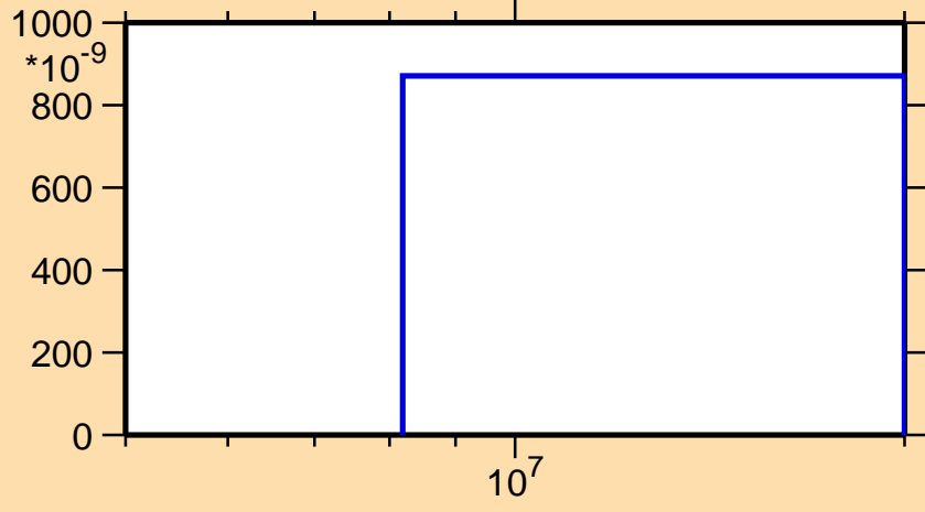
\sigma vs. E for ^{127}\text{Pm}(n,2np)
