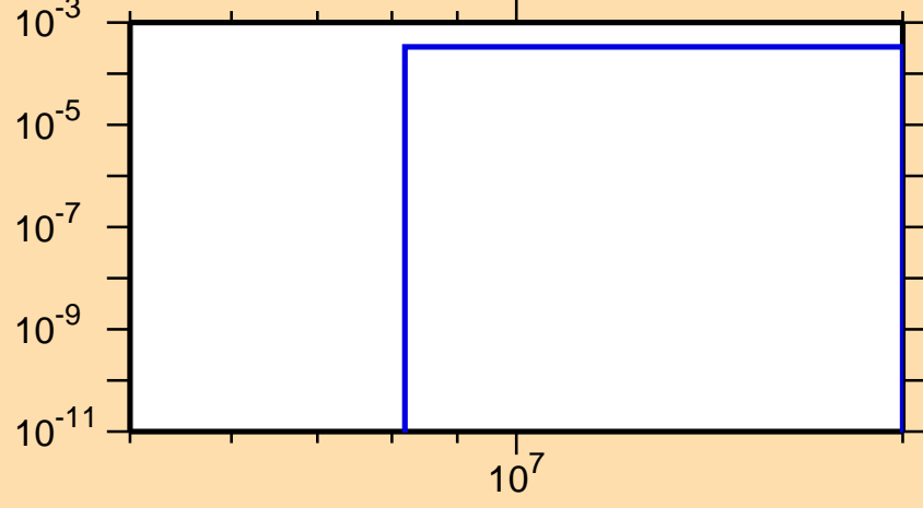
\sigma vs. E for ^{127}\text{Pm}(n,t)
