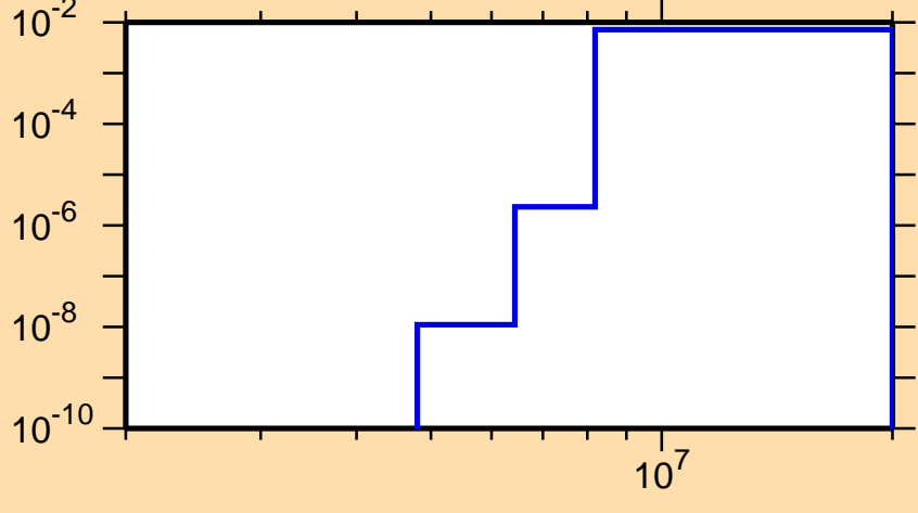
\sigma vs. E for ^{127}\text{Pm}(n,pd)
