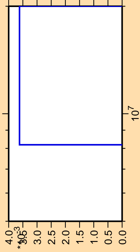
\Delta\sigma/\sigma vs. E for ^{127}\text{Pm}(n,nt)
