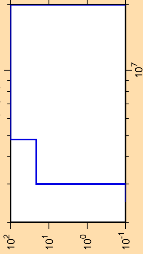
\Delta\sigma/\sigma vs. E for ^{127}\text{Pm}(n,pd)
