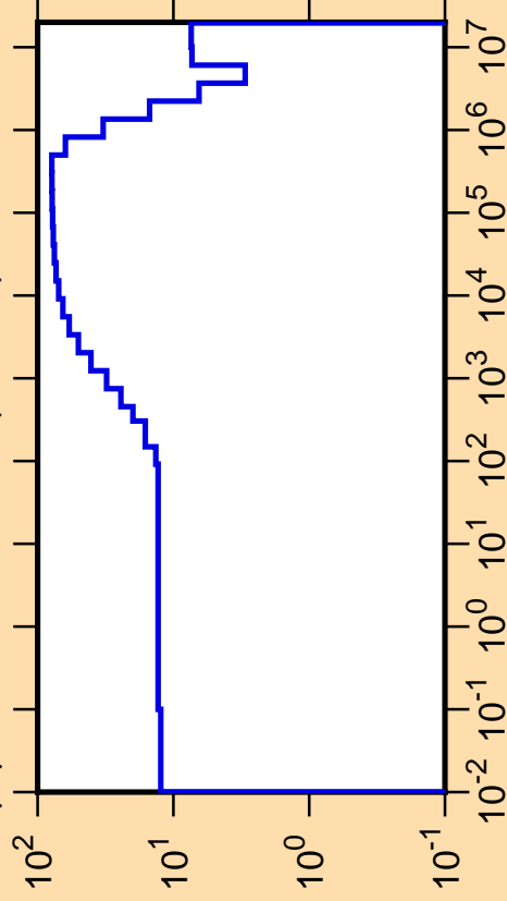
\Delta\mu/\mu vs. E for ^{128}\text{Pm}(\text{mt251})
