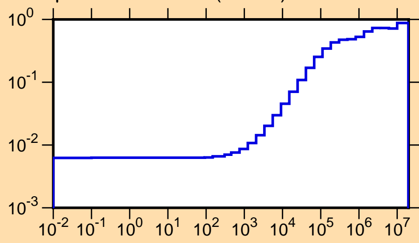
\mu vs. E for ^{128}\text{Pm}(\text{mt251})
