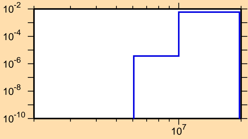
\sigma vs. E for ^{128}\text{Pm}(n,pd)
