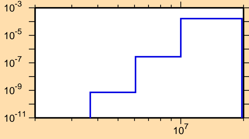
\sigma vs. E for ^{128}\text{Pm}(n,n\alpha)
