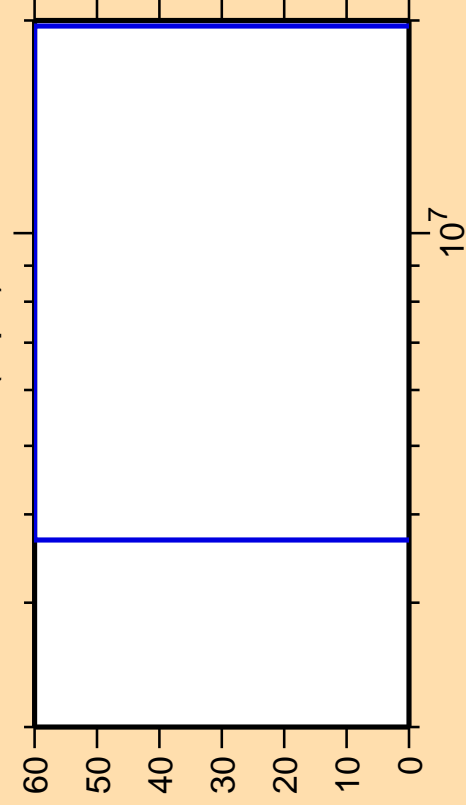
\Delta\sigma/\sigma vs. E for ^{128}\text{Pm}(n,pd)
