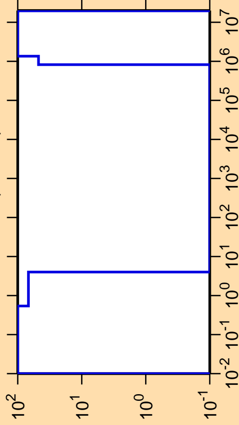
\Delta\sigma/\sigma vs. E for ^{128}\text{Pm}(n,\text{He3})
