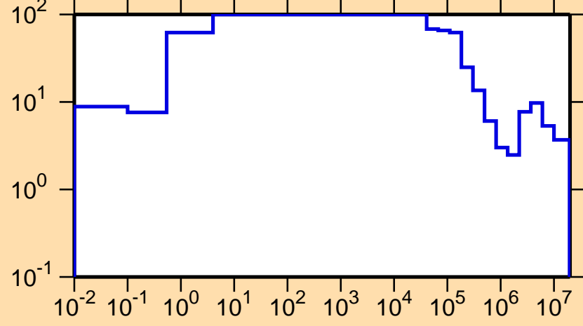
\Delta\sigma/\sigma vs. E for ^{128}\text{Pm}(n,\text{tot.})
