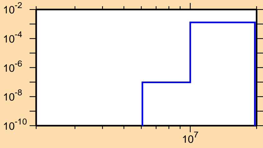
\sigma vs. E for ^{128}\text{Pm}(n,t)
