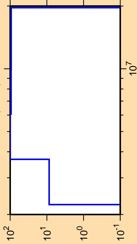
\Delta\sigma/\sigma vs. E for ^{128}\text{Pm}(n,n\alpha)
